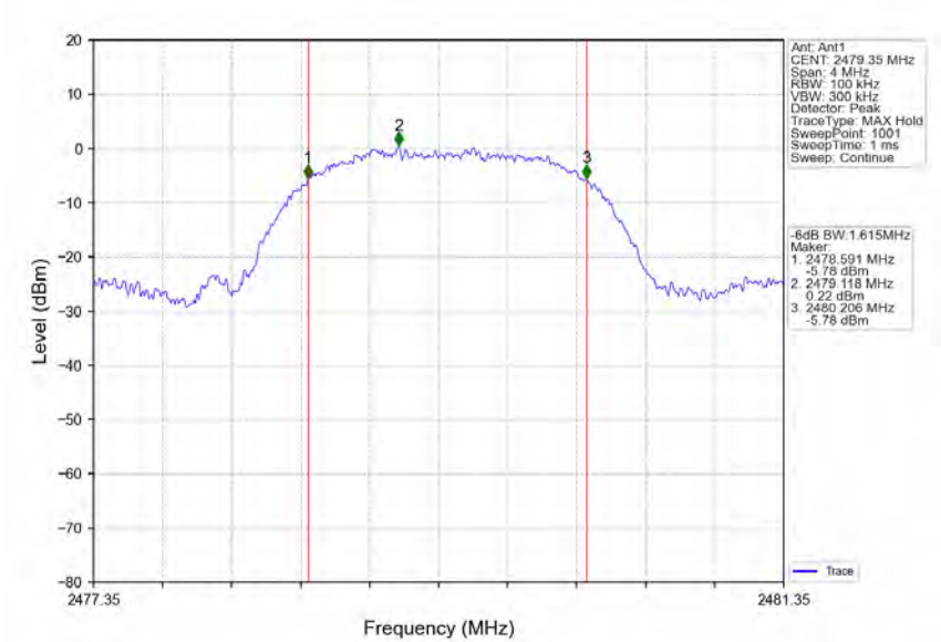
2.4G_HCH_2479.35MHz_Ant1_NTNV
