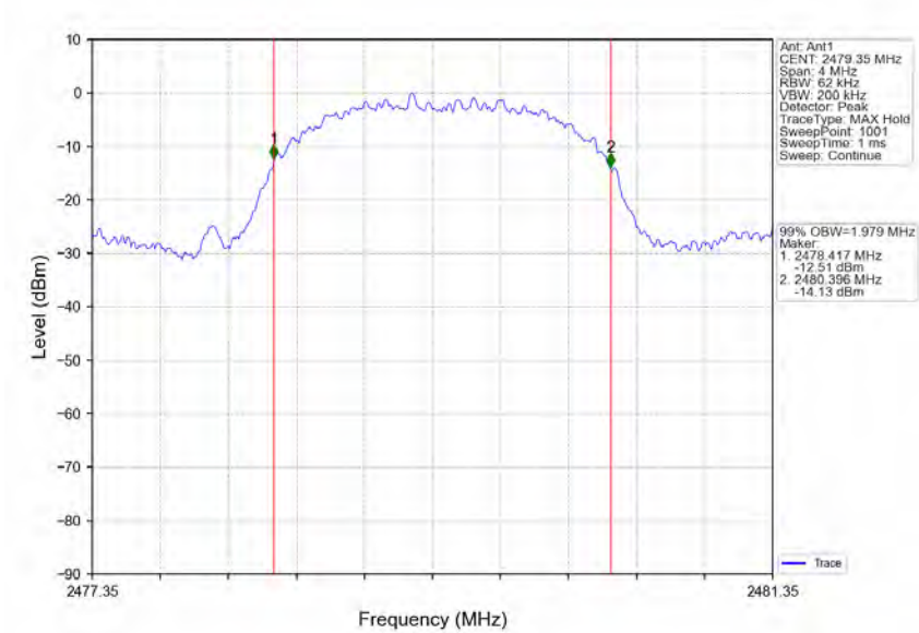
2.4G_HCH_2479.35MHz_Ant1_NTNV
