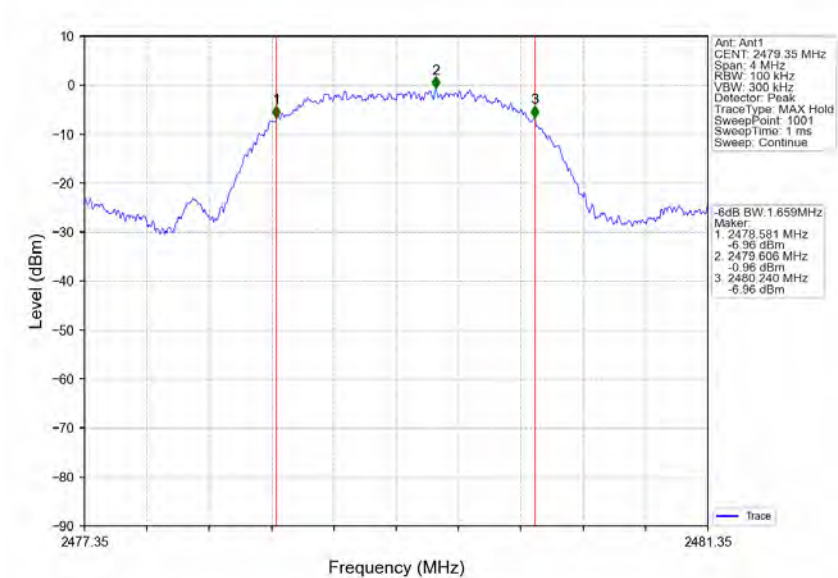
2.4G_HCH_2479.35MHz_Ant1_NTNV
