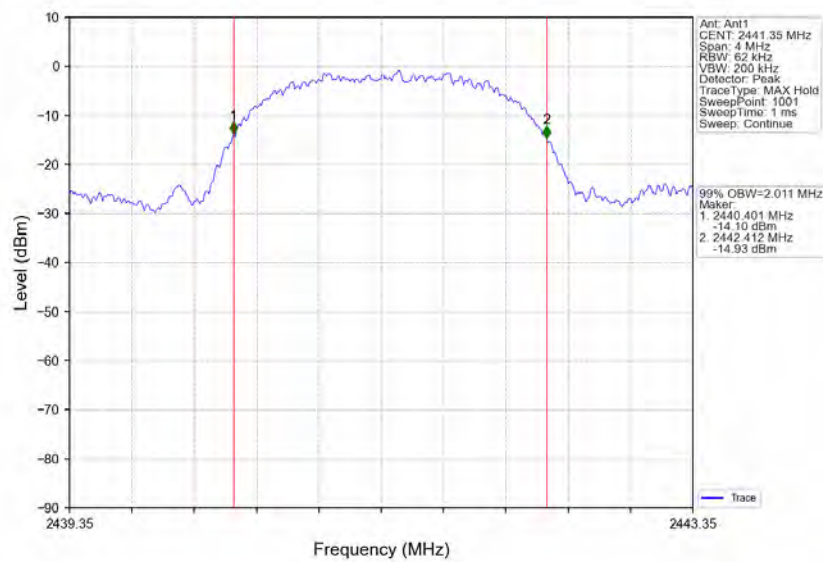
2.4G_MCH_2441.35MHz_Ant1_NTNV
