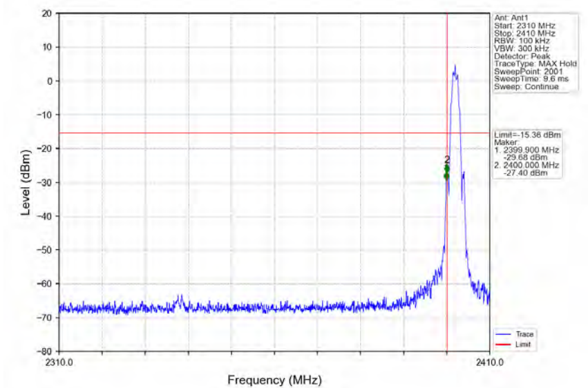
2M_LCH_2402MHz_Ant1_NTNV
