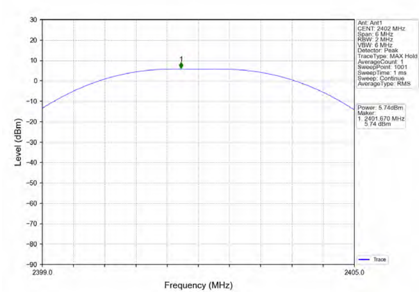
2M_LCH_2402MHz_Ant1_NTNV
