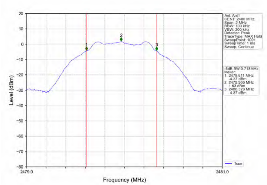
1M_HCH_2480MHz_Ant1_NTNV
