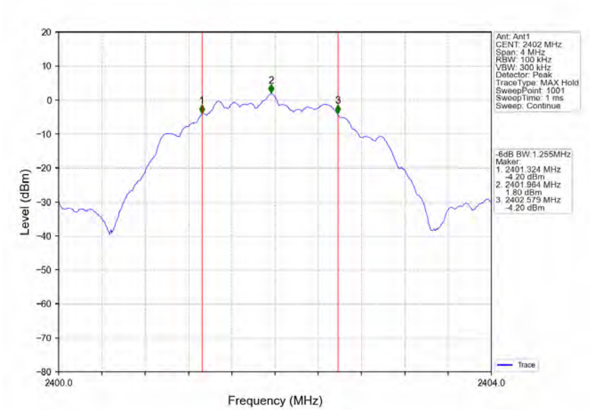
2M_LCH_2402MHz_Ant1_NTNV
