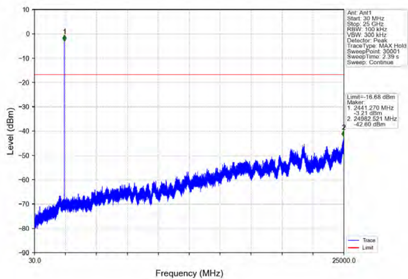
Pi/4DQPSK_2DH5_MCH_2441MHz_Ant1_NTNV
