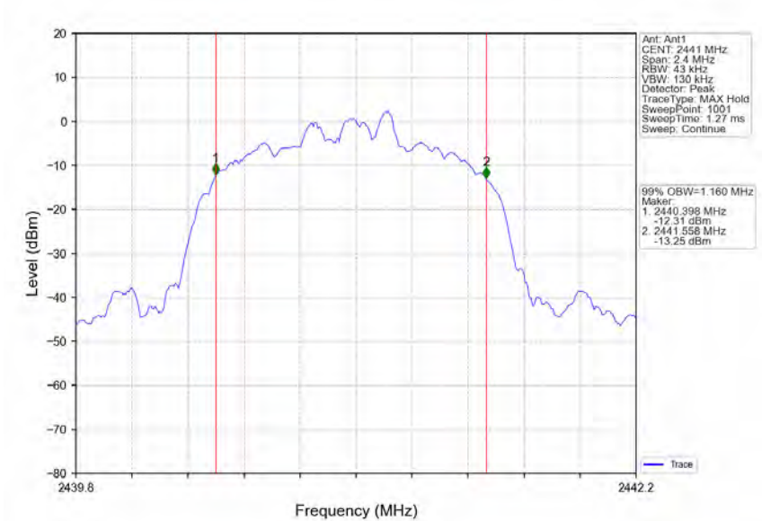
8DPSK_3DH5_MCH_2441MHz_Ant1_NTNV
