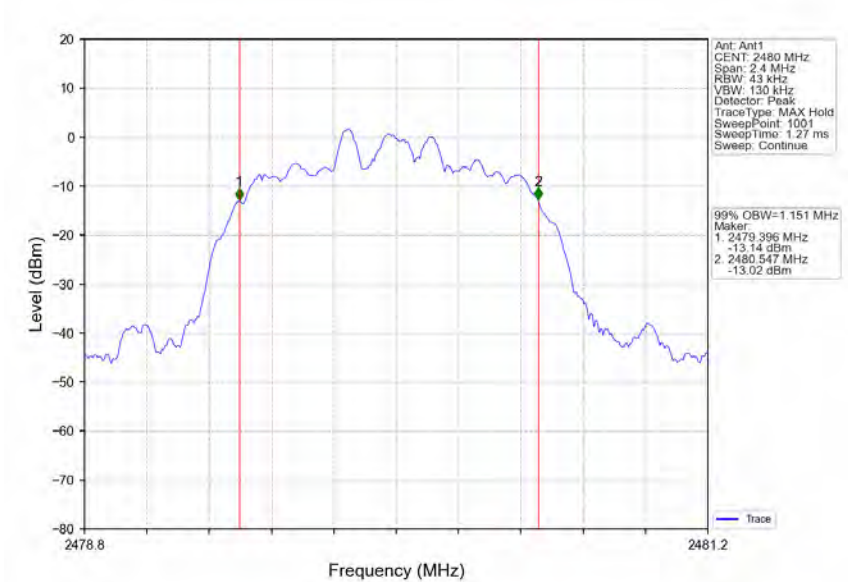
Pi/4DQPSK_2DH5_HCH_2480MHz_Ant1_NTNV
