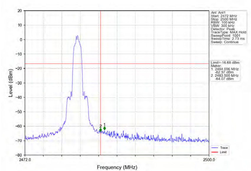
Pi/4DQPSK_2DH5_HCH_2480MHz_Ant1_NTNV
