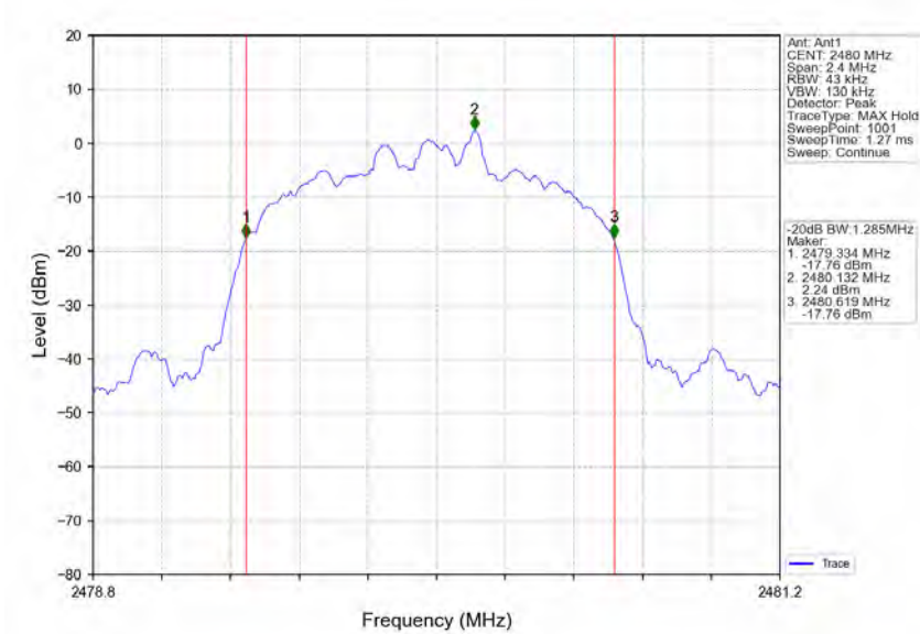
8DPSK_3DH5_HCH_2480MHz_Ant1_NTNV
