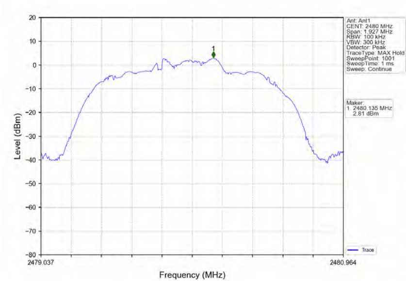
8DPSK_3DH5_HCH_2480MHz_Ant1_NTNV
