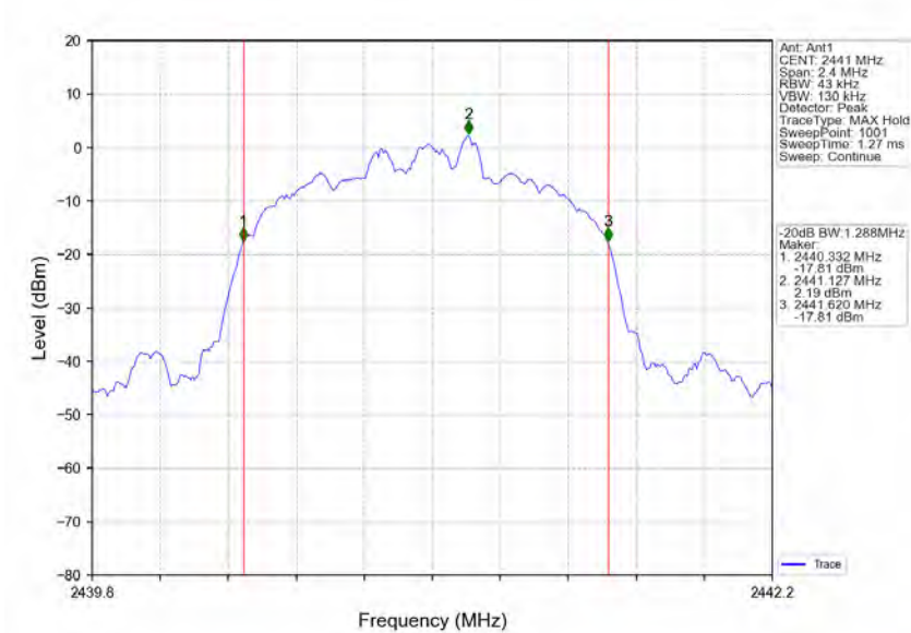
8DPSK_3DH5_MCH_2441MHz_Ant1_NTNV
