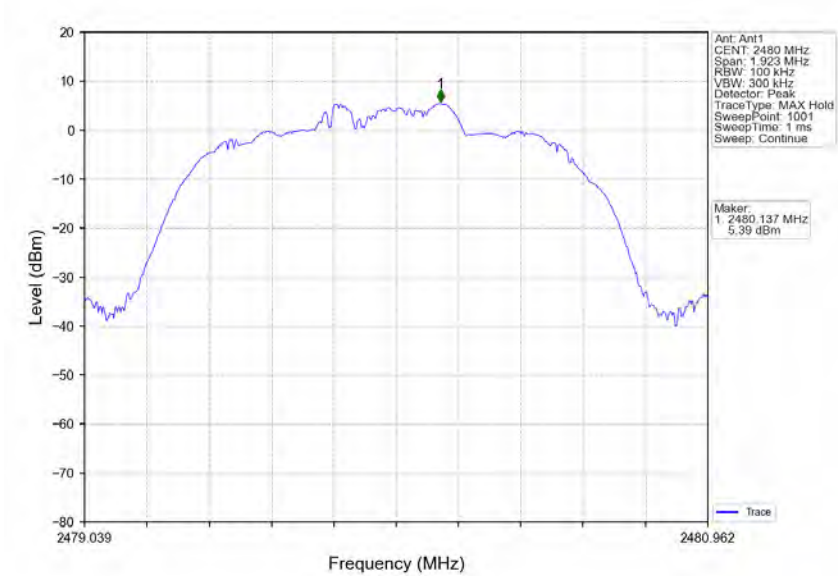
8DPSK_3DH5_HCH_2480MHz_Ant1_NTNV
