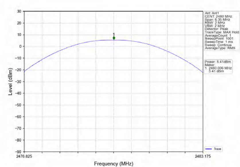
Pi/4DQPSK_2DH5_HCH_2480MHz_Ant1_NTNV
