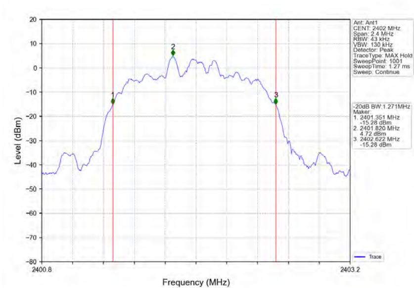
Pi/4DQPSK_2DH5_LCH_2402MHz_Ant1_NTNV
