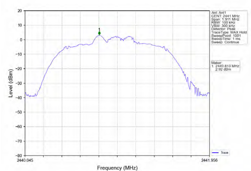
Pi/4DQPSK_2DH5_MCH_2441MHz_Ant1_NTNV
