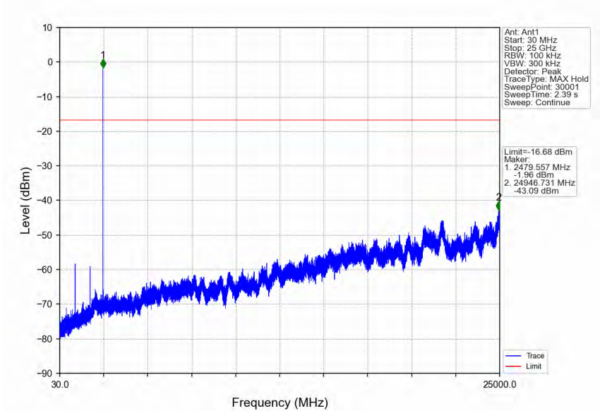
Pi/4DQPSK_2DH5_HCH_2480MHz_Ant1_NTNV
