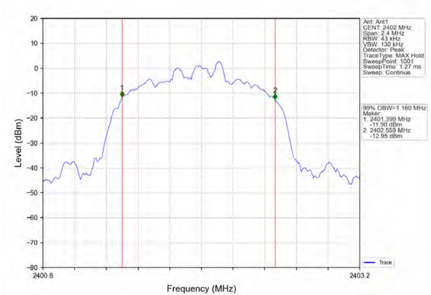
8DPSK_3DH5_LCH_2402MHz_Ant1_NTNV
