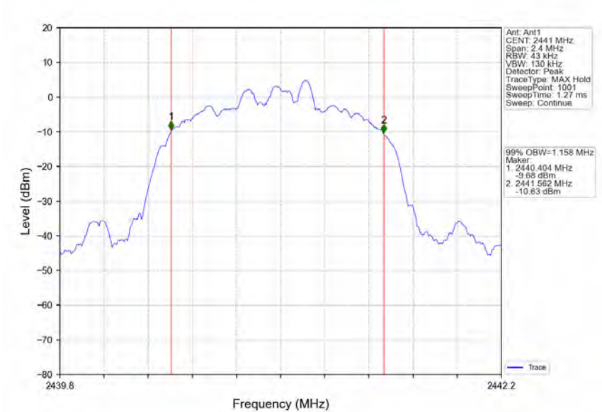
8DPSK_3DH5_MCH_2441MHz_Ant1_NTNV
