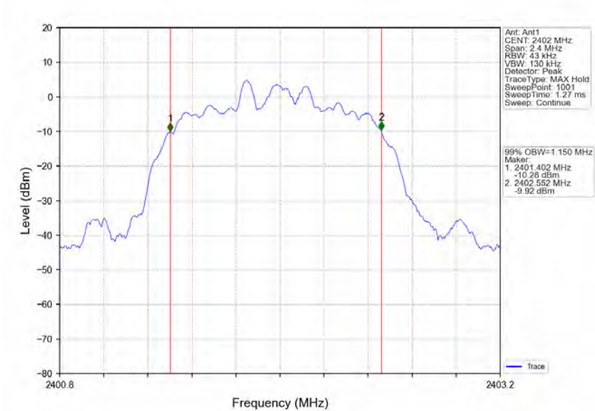
Pi/4DQPSK_2DH5_LCH_2402MHz_Ant1_NTNV
