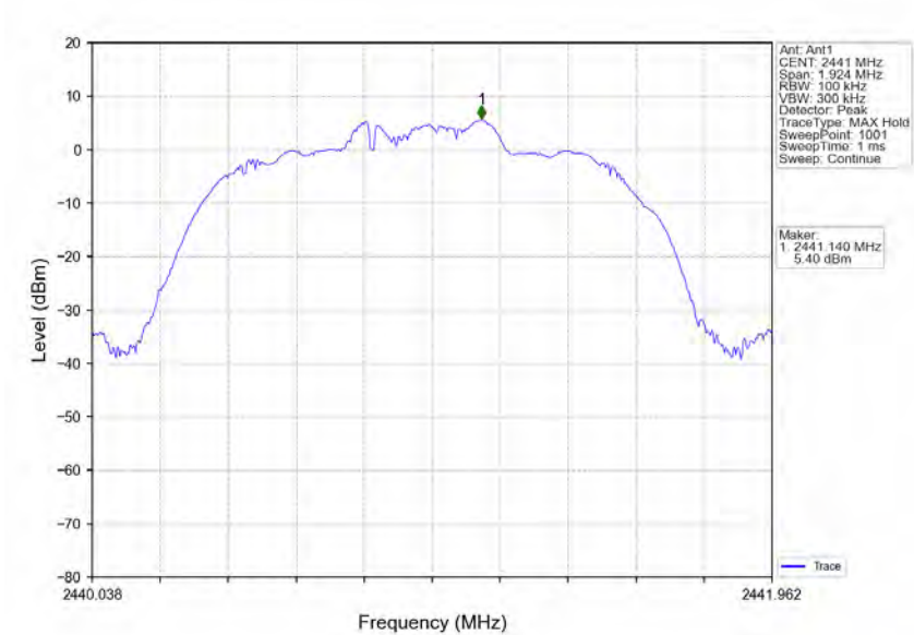
8DPSK_3DH5_MCH_2441MHz_Ant1_NTNV
