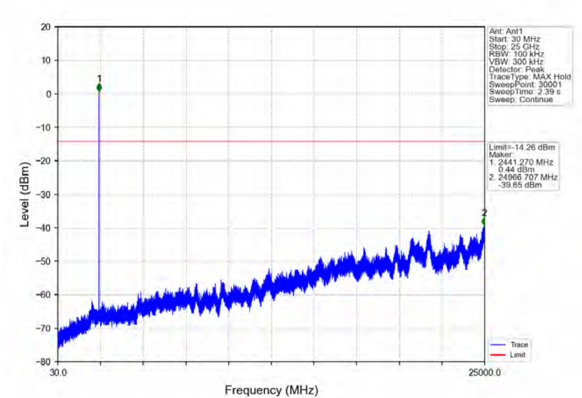
Pi/4DQPSK_2DH5_MCH_2441MHz_Ant1_NTNV
