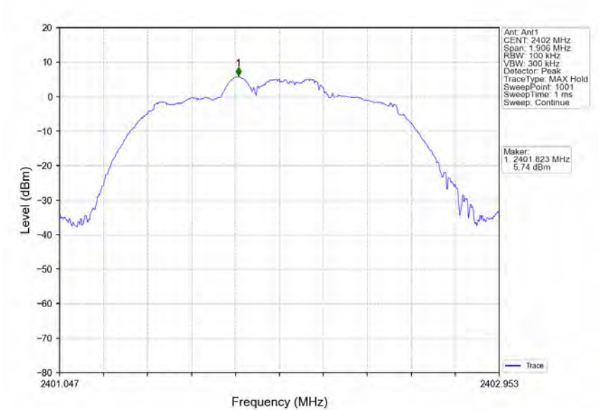
Pi/4DQPSK_2DH5_LCH_2402MHz_Ant1_NTNV
