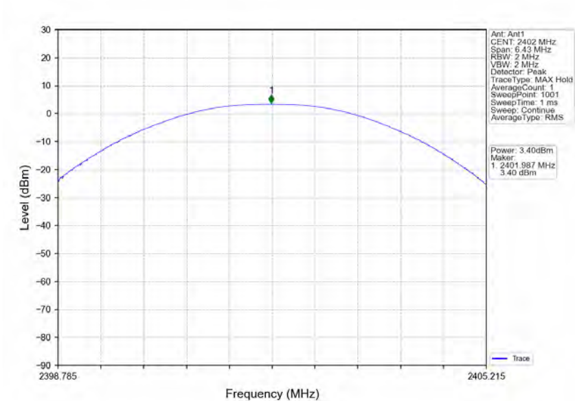
8DPSK_3DH5_LCH_2402MHz_Ant1_NTNV
