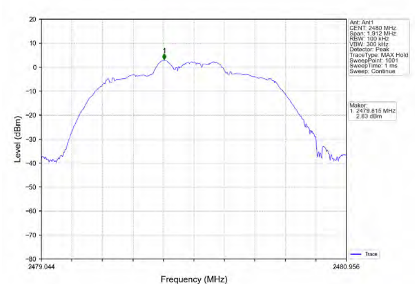
Pi/4DQPSK_2DH5_HCH_2480MHz_Ant1_NTNV
