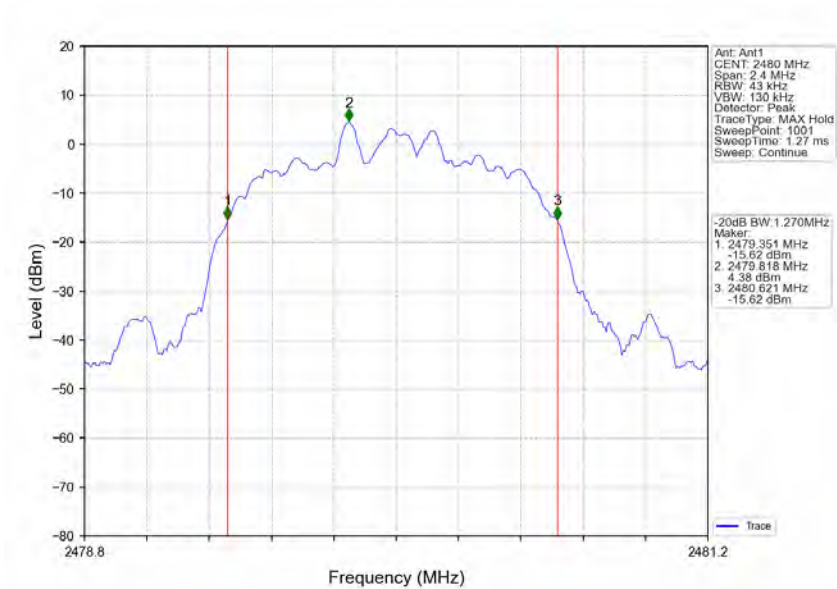
Pi/4DQPSK_2DH5_HCH_2480MHz_Ant1_NTNV
