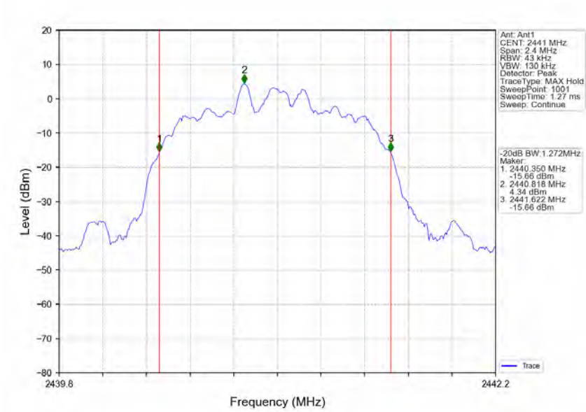
Pi/4DQPSK_2DH5_MCH_2441MHz_Ant1_NTNV
