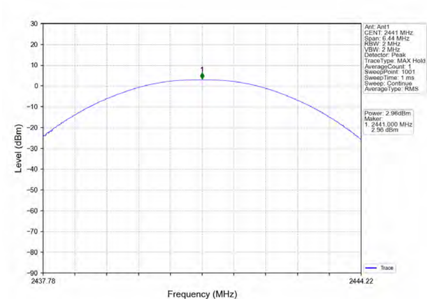
8DPSK_3DH5_MCH_2441MHz_Ant1_NTNV
