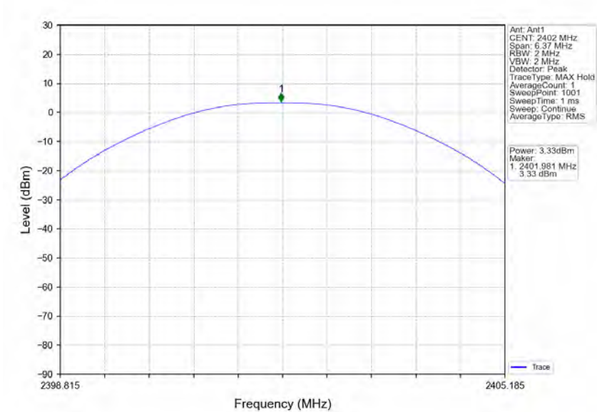
Pi/4DQPSK_2DH5_LCH_2402MHz_Ant1_NTNV
