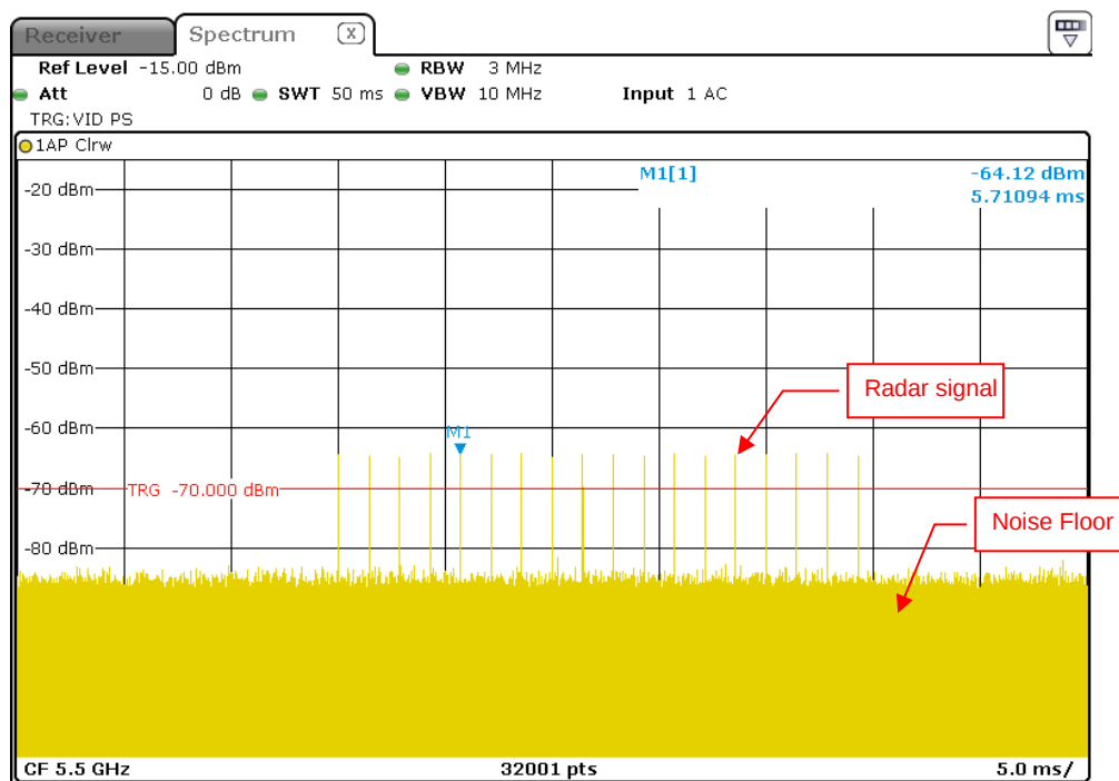
Radar Signal 0
