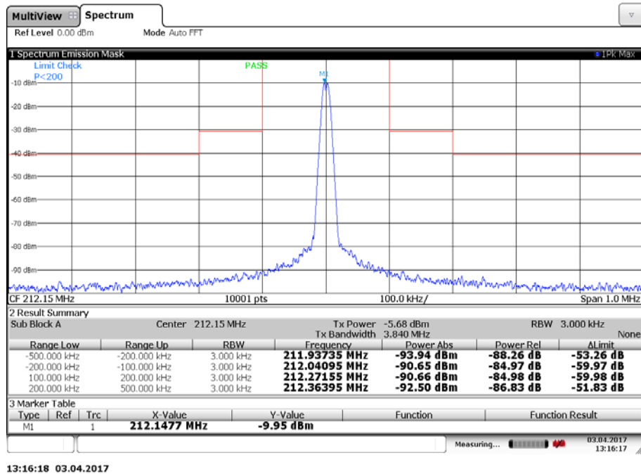
Plot 6: 212.150 MHz, spectrum mask
