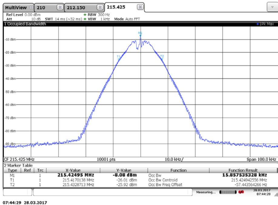
Plot 3: 215.425 MHz, max hold with frequency variation from 50 Hz to 15 kHz
