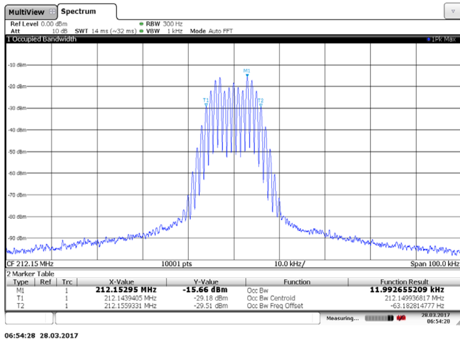
Plot 2: 212.150 MHz, 1 kHz tone
