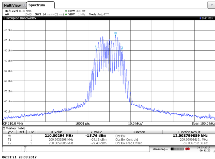
Plot 1: 210.000 MHz, 1 kHz tone
