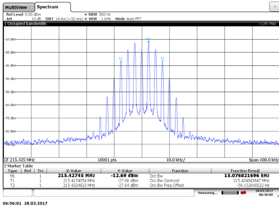
Plot 6: 215.425 MHz, 2.5 kHz tone
