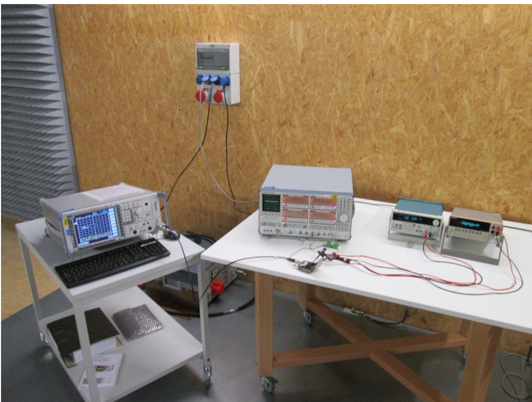
Test Setup: Frequency stability measurement
