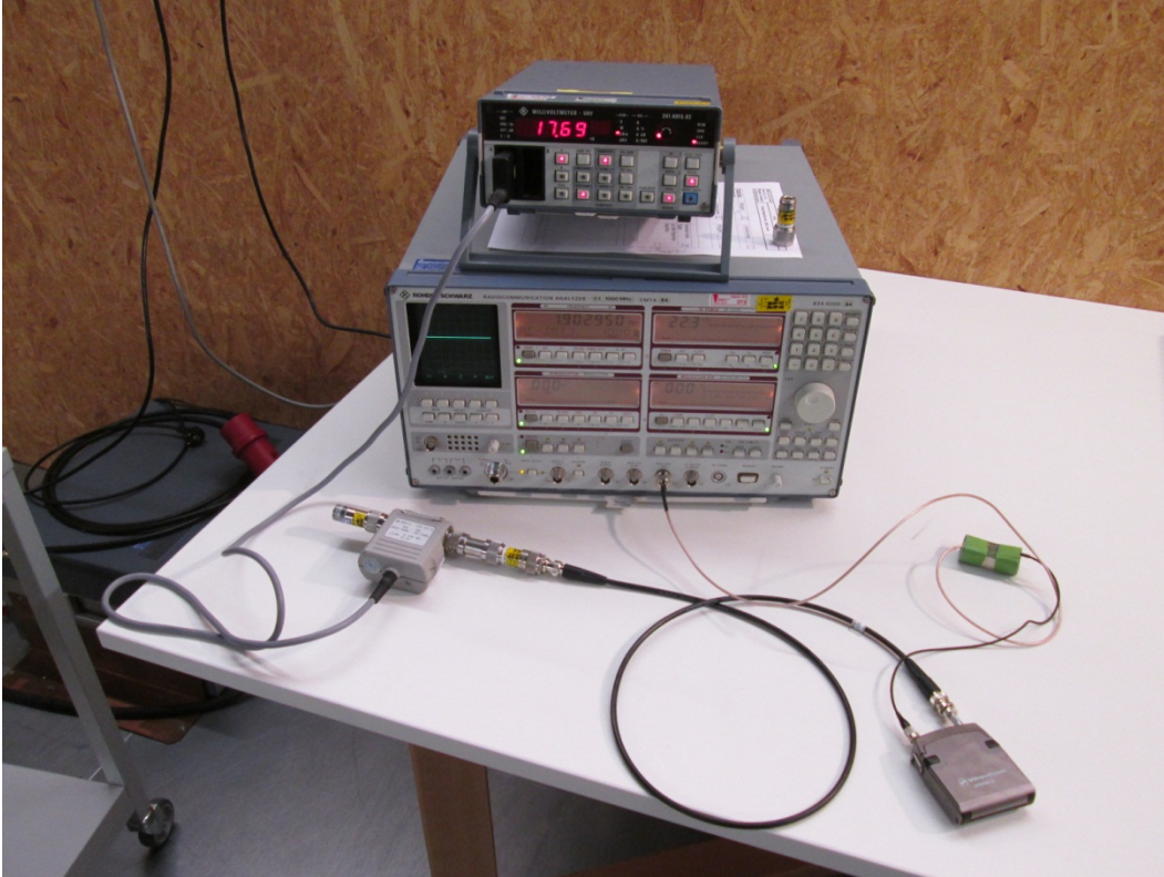
Test Setup: TX power measurement
