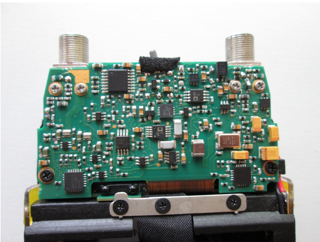
Main board of EUT #T1541593, bottom
