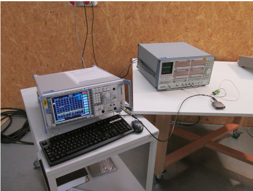
Test Setup: Emission bandwidth measurement
