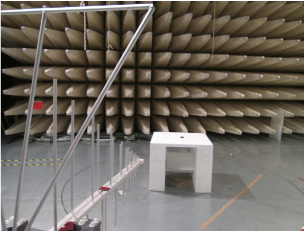
Test Setup: Field strength of spurious radiation measurement
