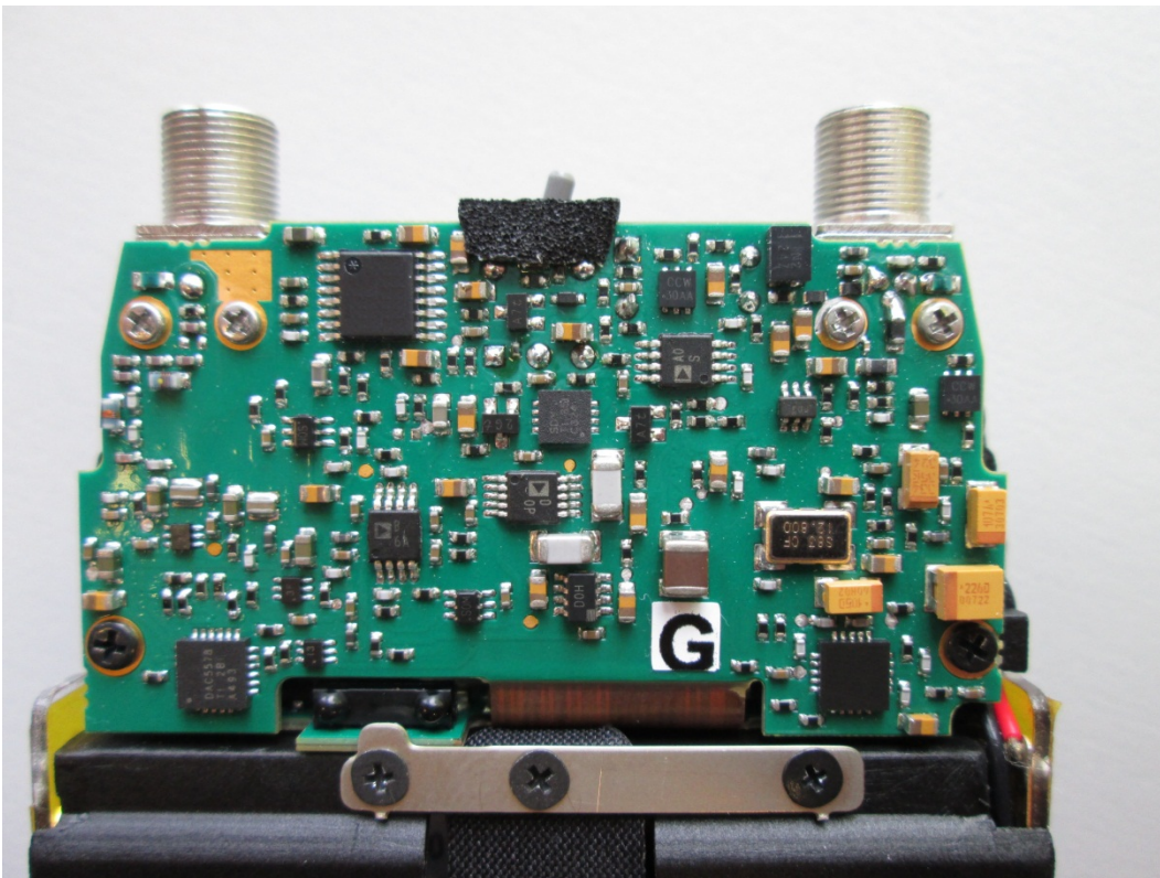
Main board of EUT #T1541595, bottom
