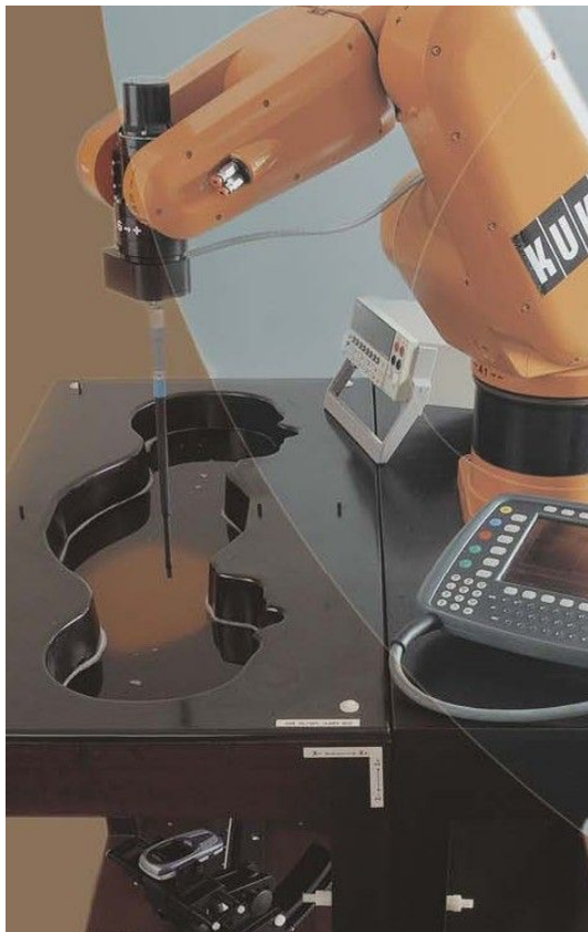
Picture A - SAR Dosimetric Assessment System
