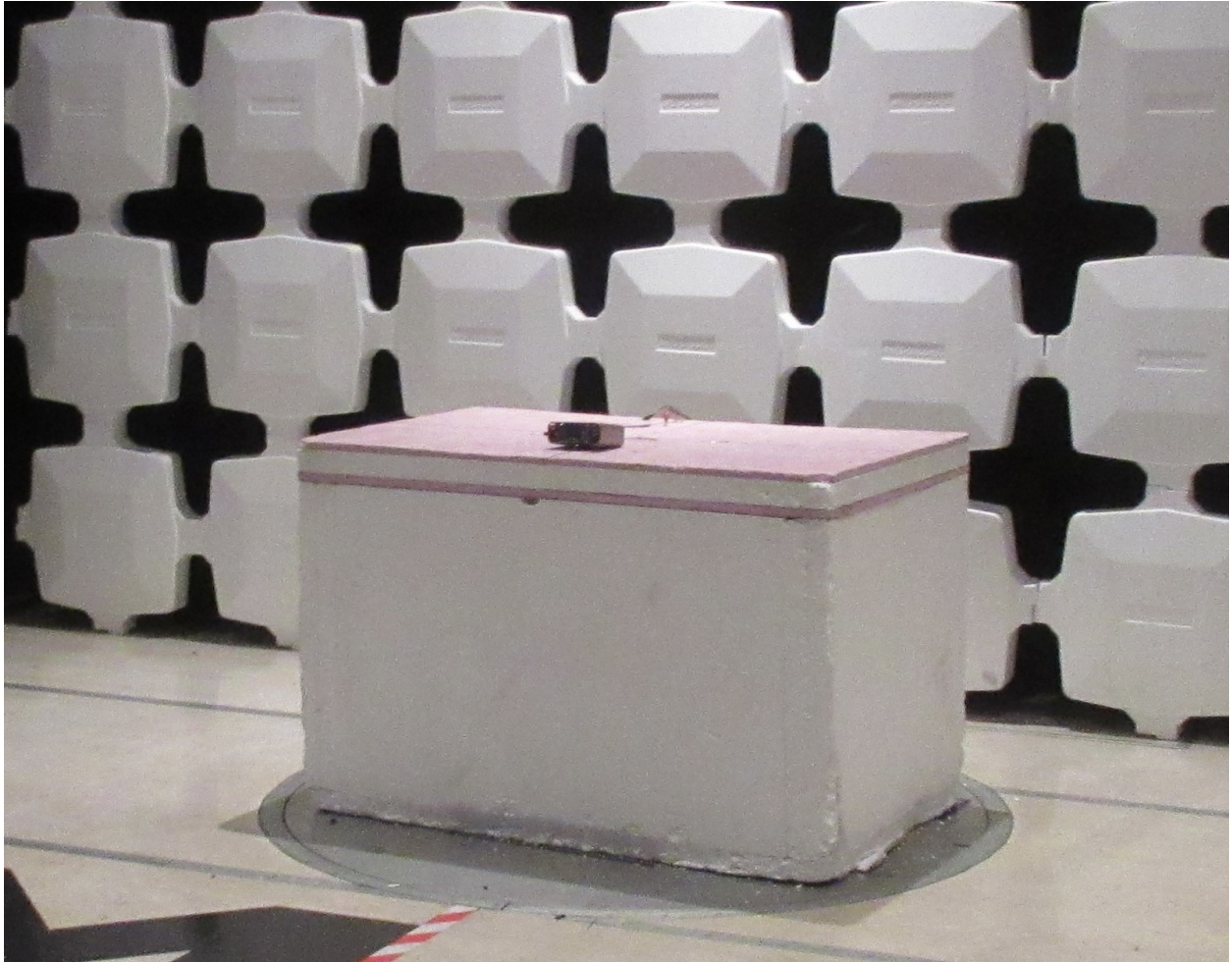
Radiated Testing, Table Setup #1
