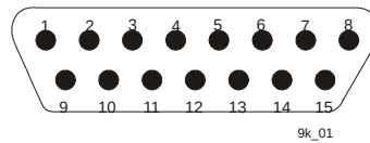
DB15(M) Plug (view looking into transceiver)
