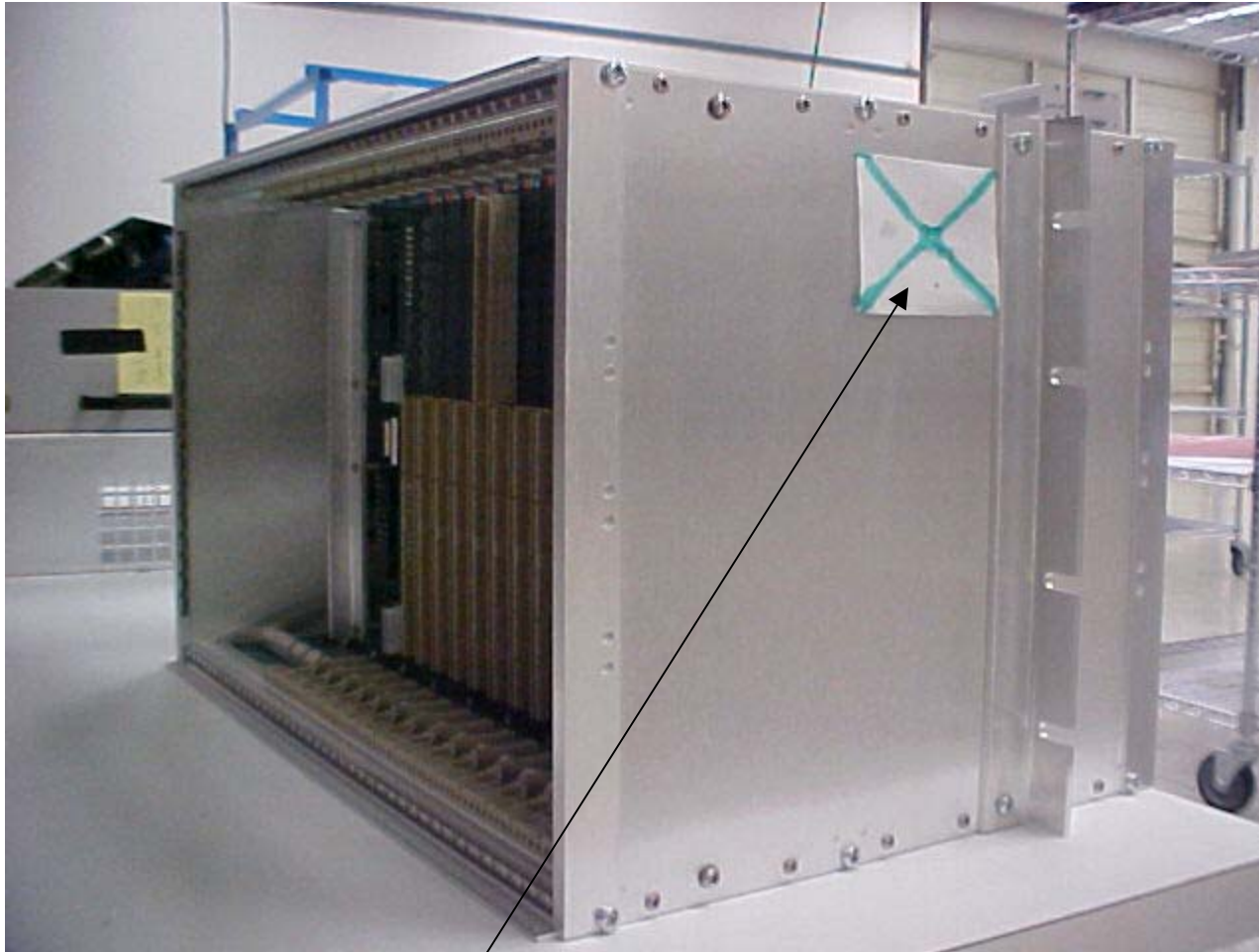
FCC ID Location on the amplifier rack (View is the front of the rack)
