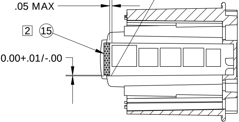
SECTION A-A PLACEMENT OF ITEM 15
