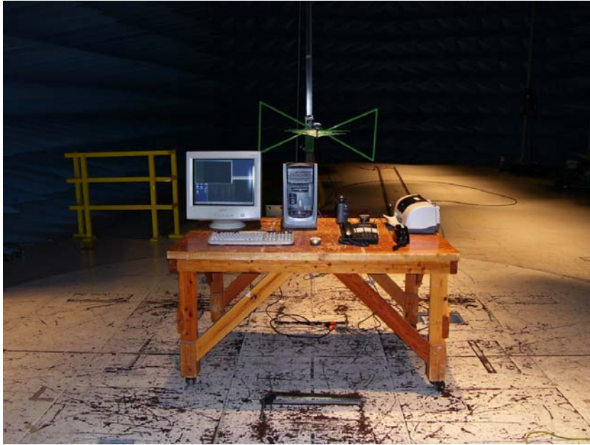
Photograph 4. Radiated Emission Limits Test Setup, 30 MHz to 1 GHz, Front View
