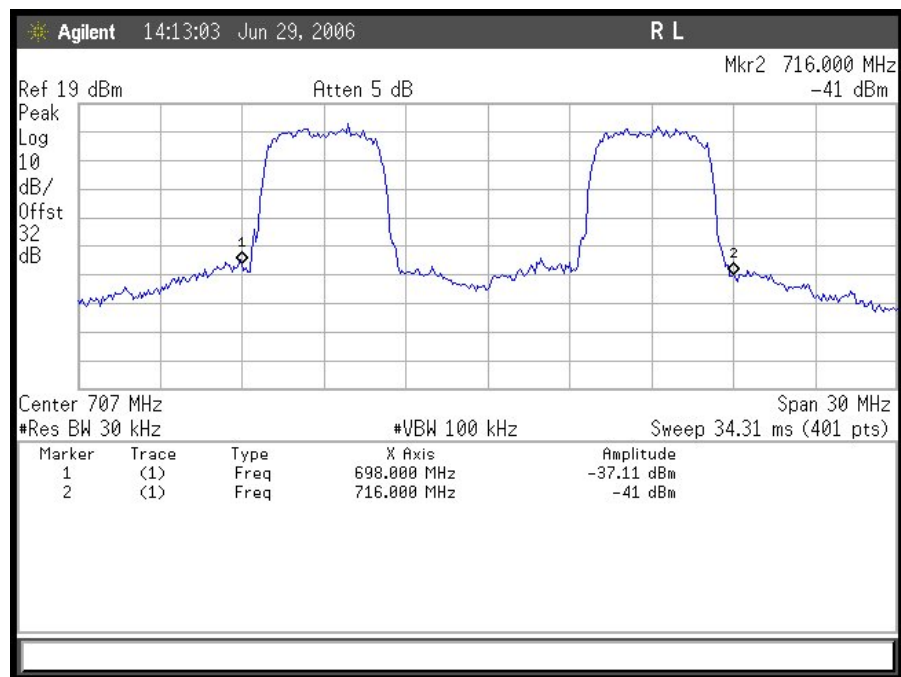
Plot 16. Frequency stability at +10 deg C and normal voltage
