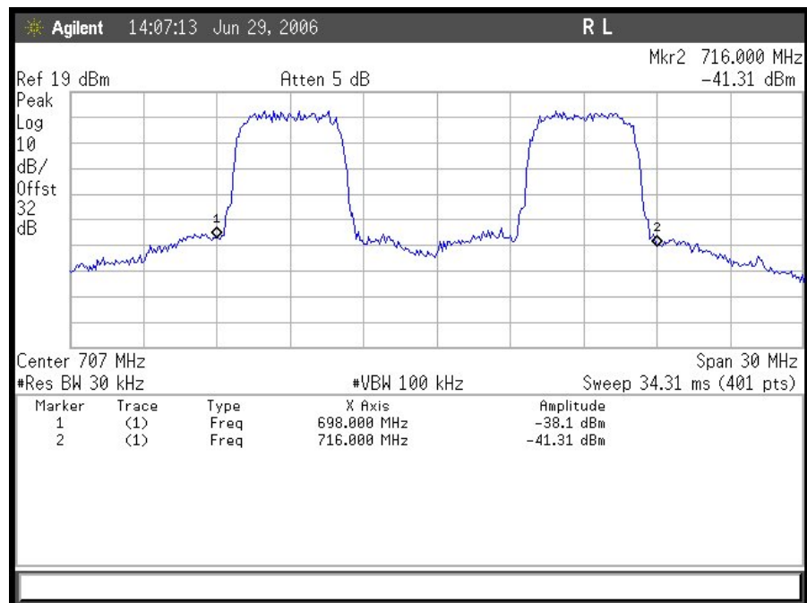
Plot 12. Frequency stability at 0 deg C and normal voltage
