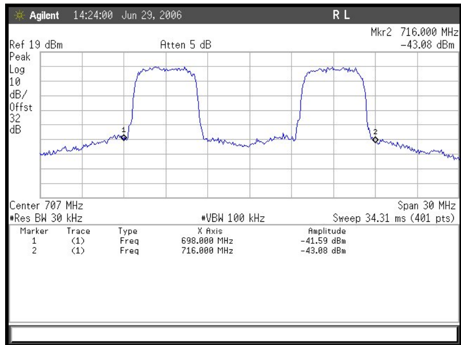
Plot 15. Frequency stability at 20 deg C and maximum voltage
