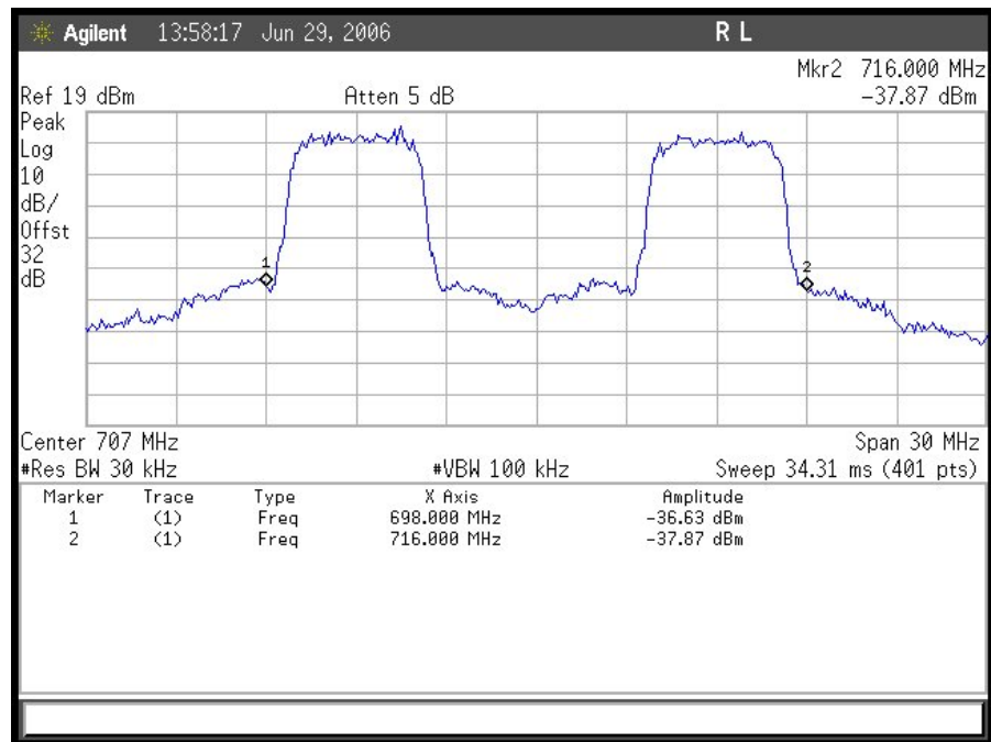
Plot 11. Frequency stability at -10 deg C and normal voltage
