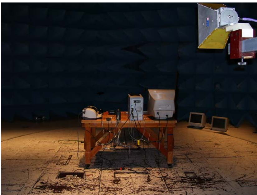
Photograph 7. Radiated Emission Limits Test Setup, 1 GHz to 2 GHz, Back View
