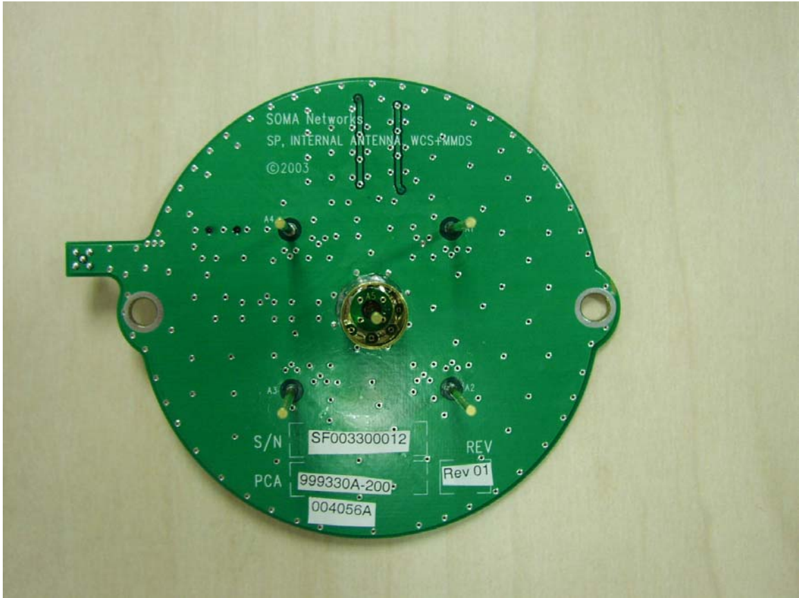
Internal Antenna (Component Side)
