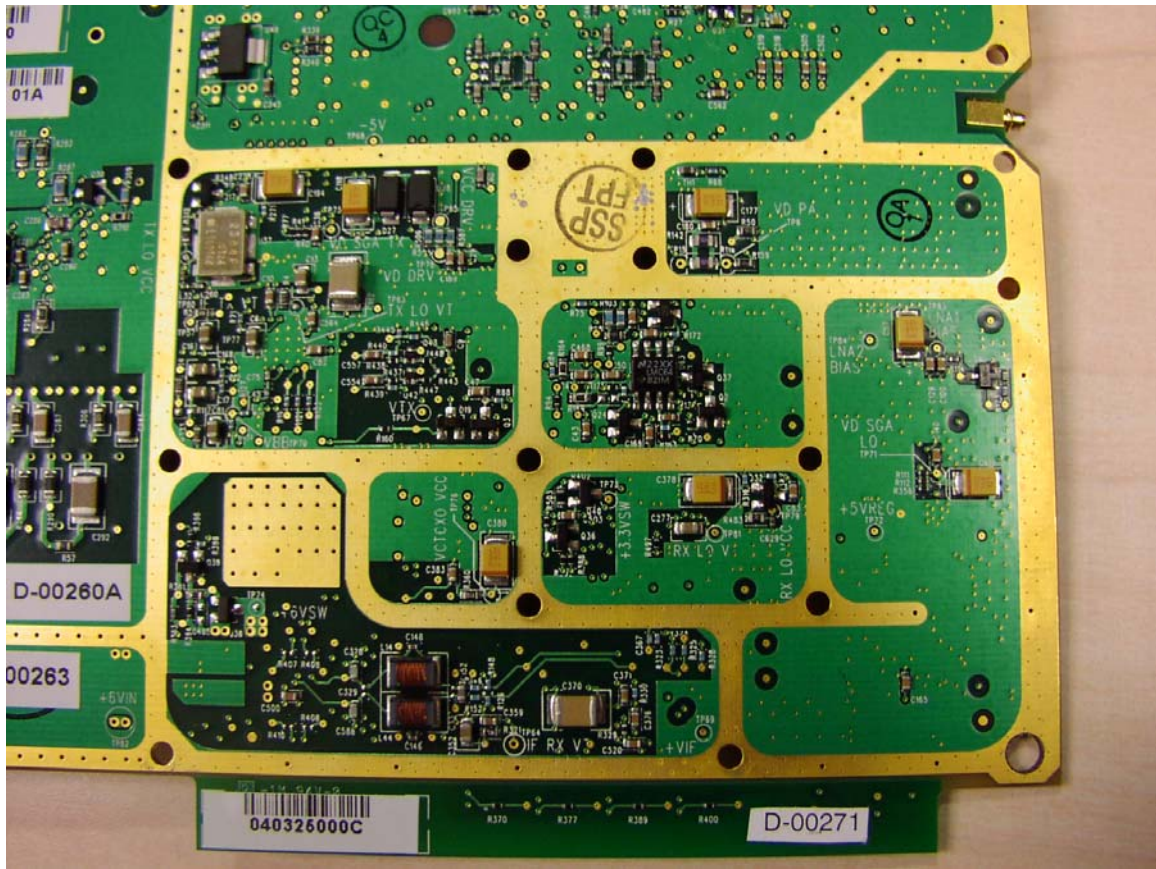
RF Portion Back Side
