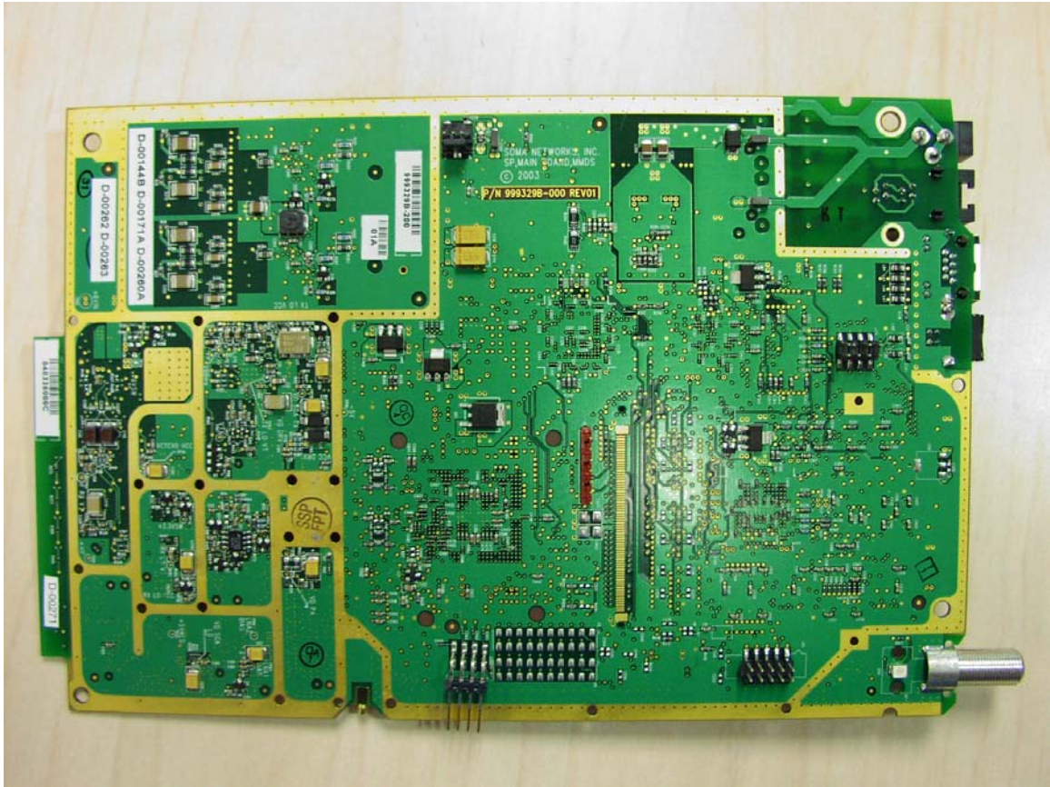
Back side no shield
