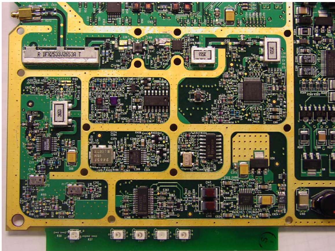
RF portion Front side
