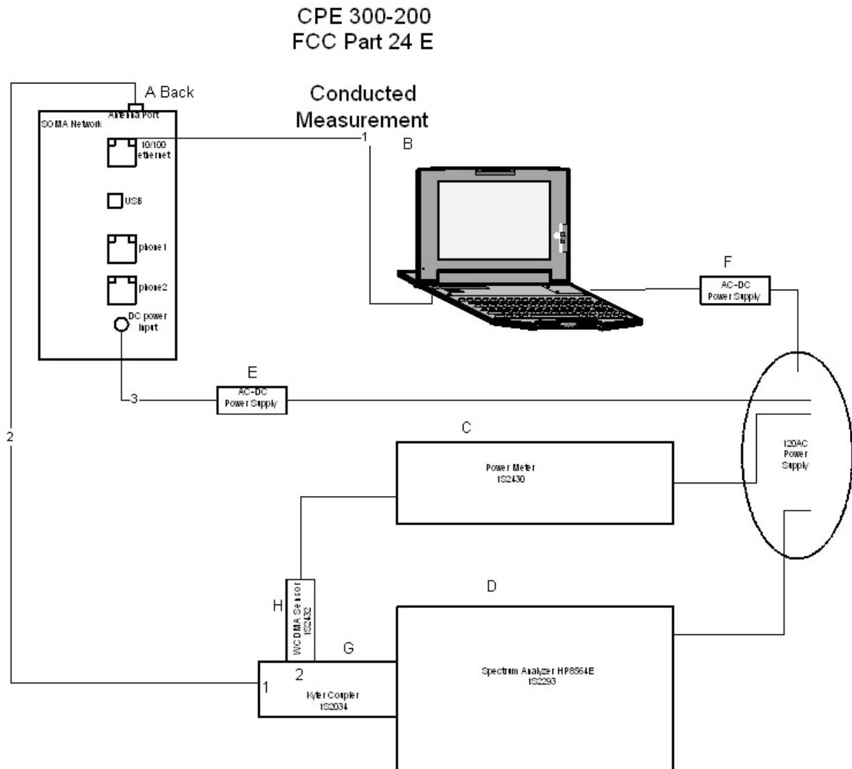
Figure 1. Block Diagram of Test Configuration (Conducted Measurement)
