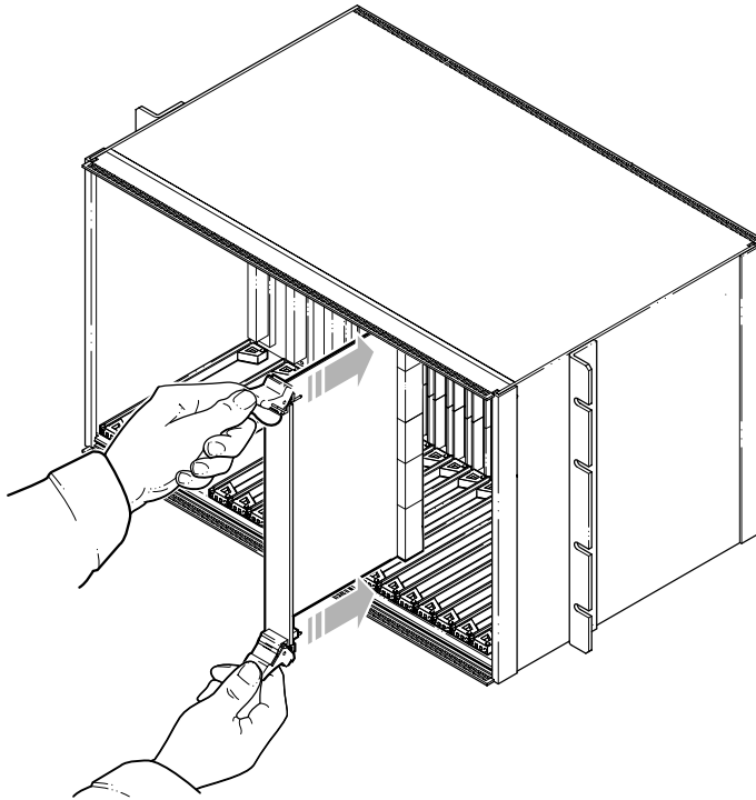
Figure 4.15 Card Insertion
