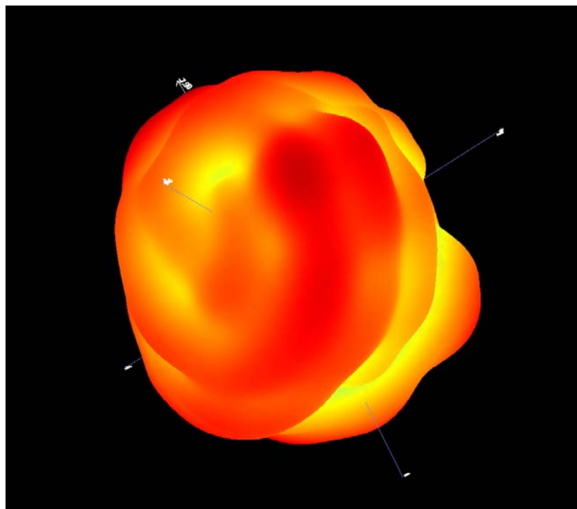
B1.2 3D Pattern for 2450MHz
