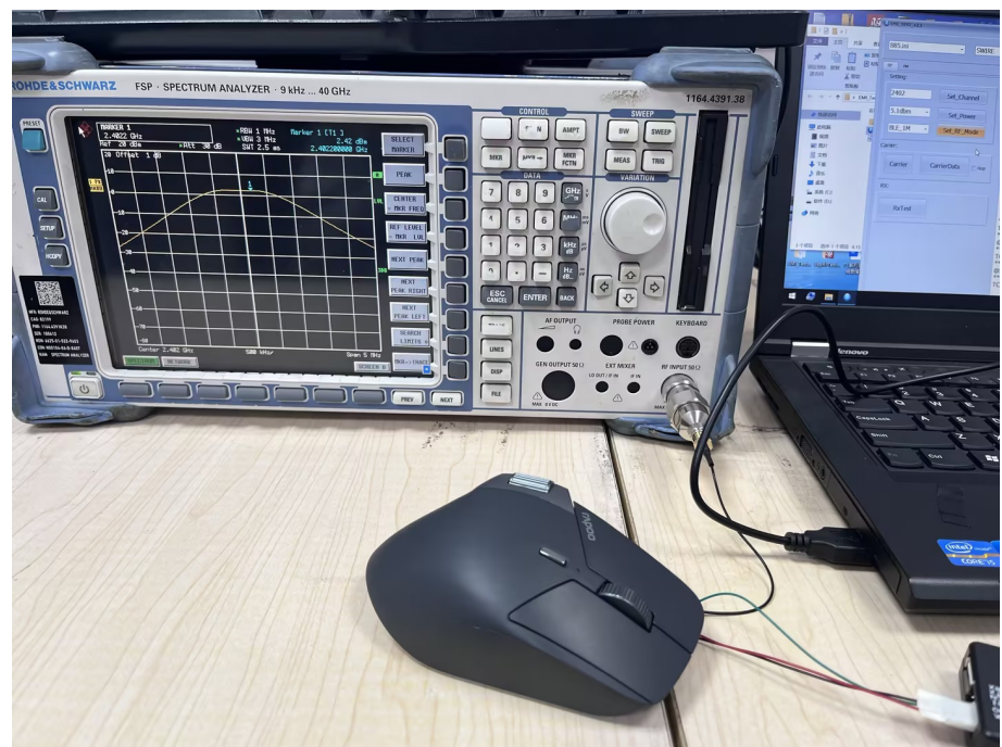
Radio Test Setup View (LE)
