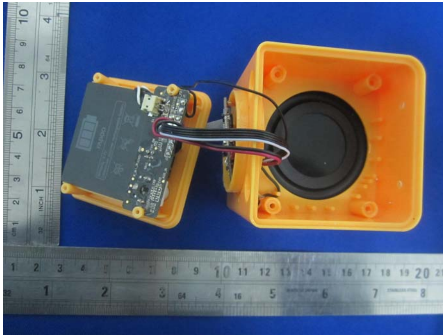
EUT –Rear Uncover View
