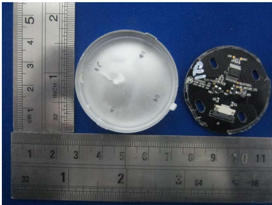
EUT –Control Board Off View
