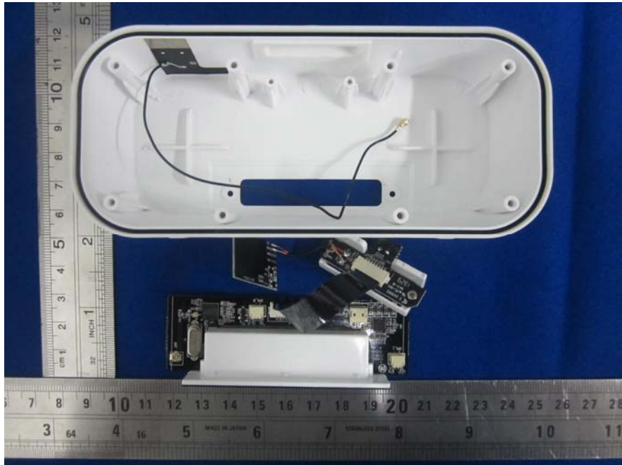
EUT –All Board Off View
