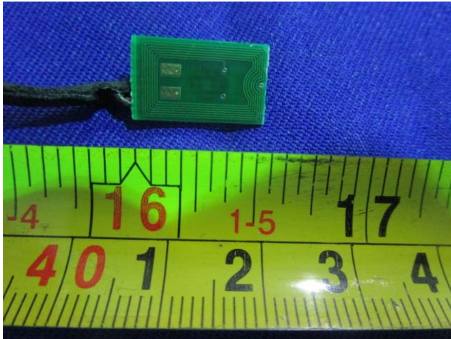
EUT –NFC Board
