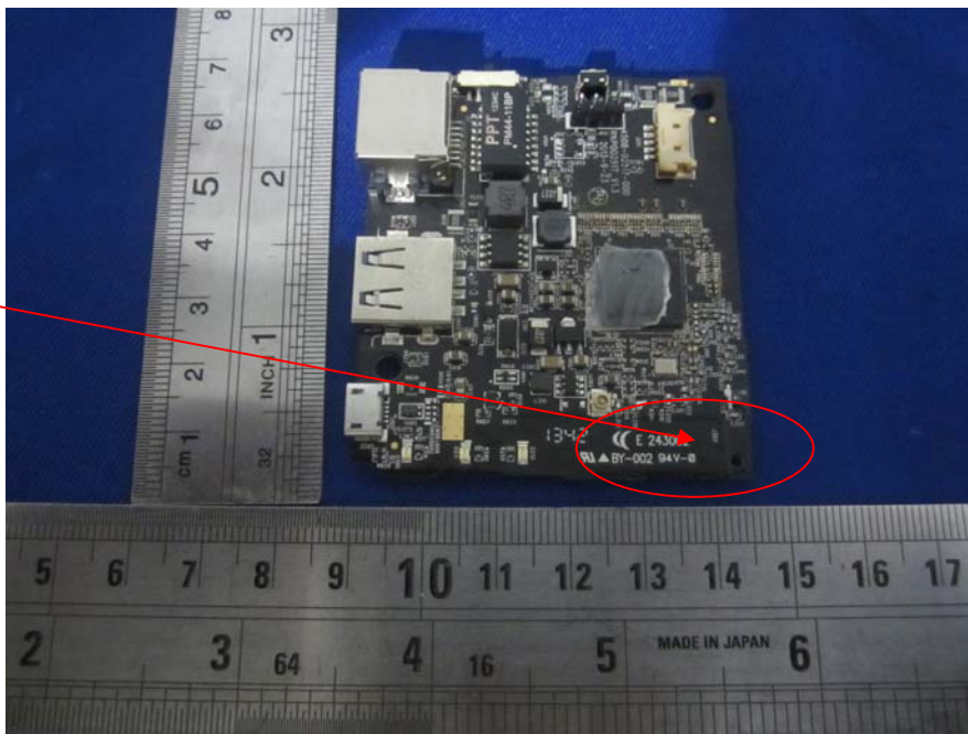
EUT –Antenna View View
