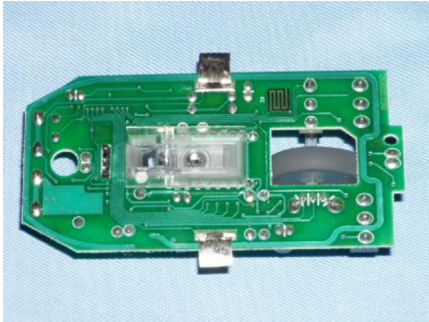
(5) Main board solder side
