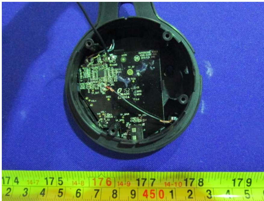
EUT –Left Uncover View
