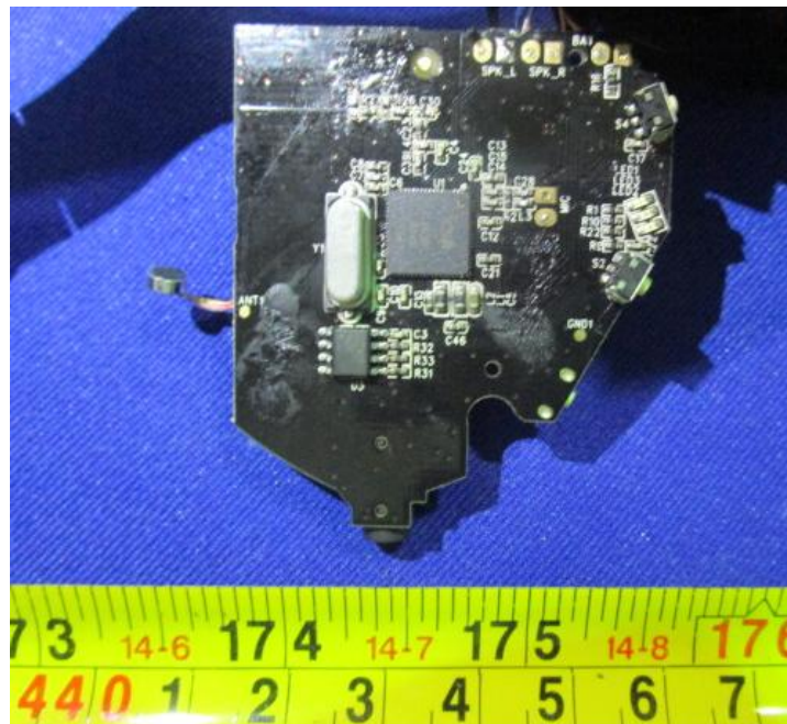
EUT–Main Board Bottom View
