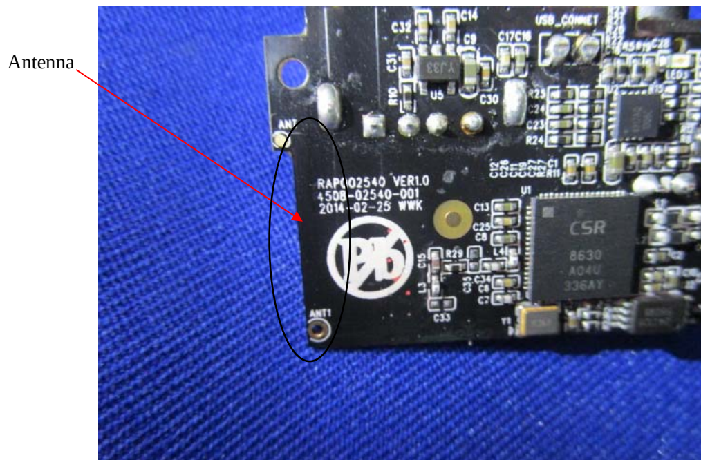
EUT – RF Chip and Antenna View
