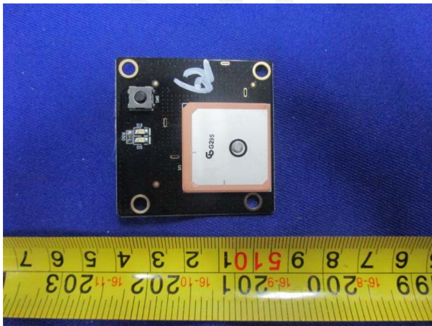
EUT –GPS Module Bottom & GPS Antenna View
