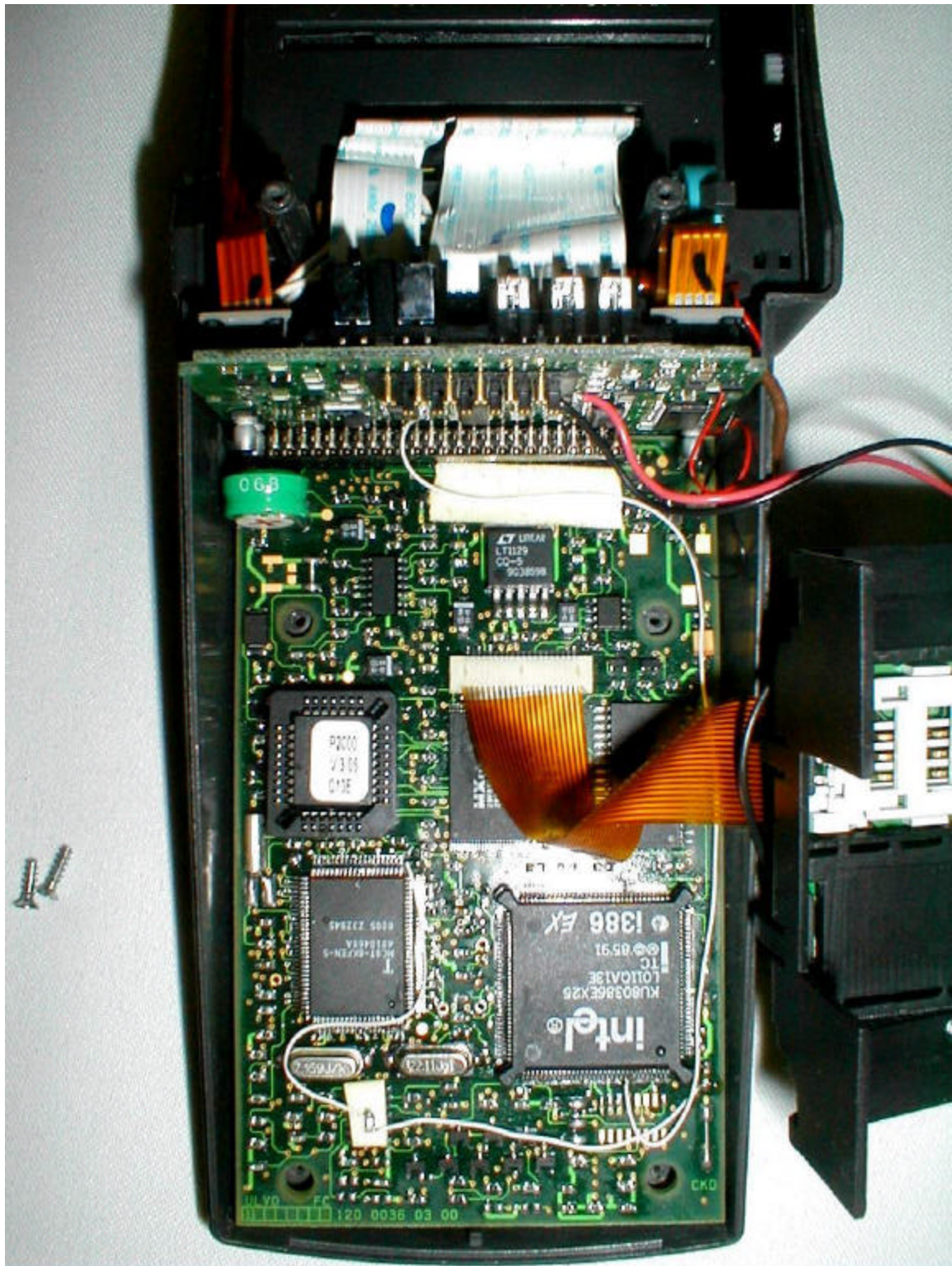
Lower Cover Removed
