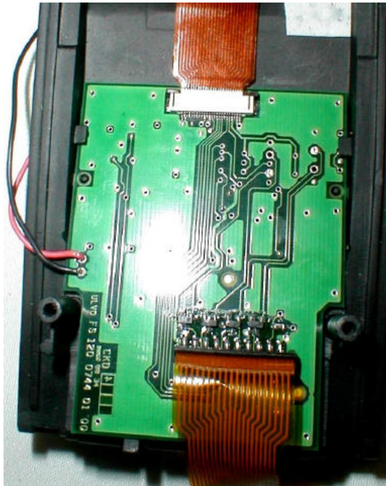
Power PCB
