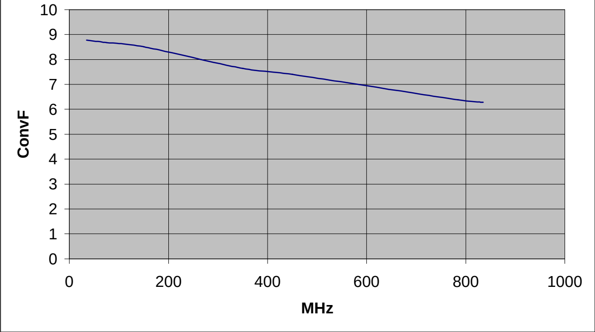
Probe Conversion Factor Vesus Frequency
