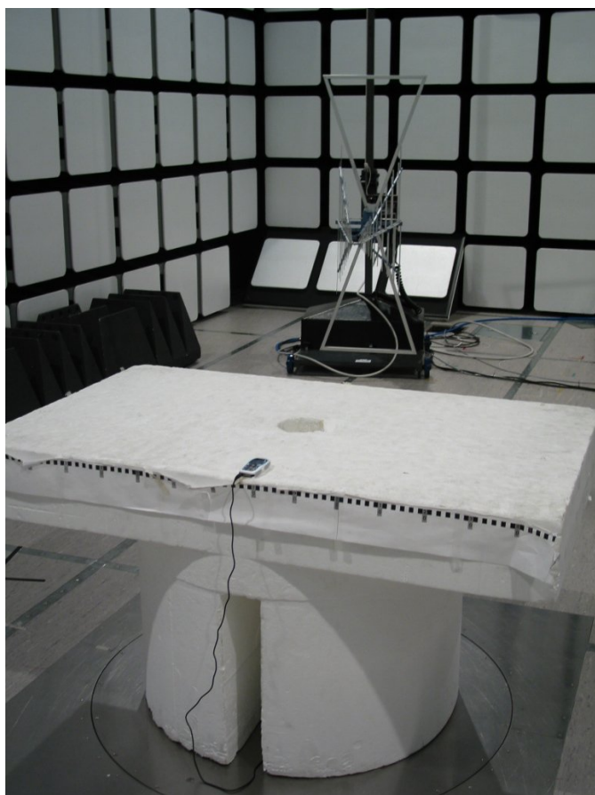
Radiated emission measurement
