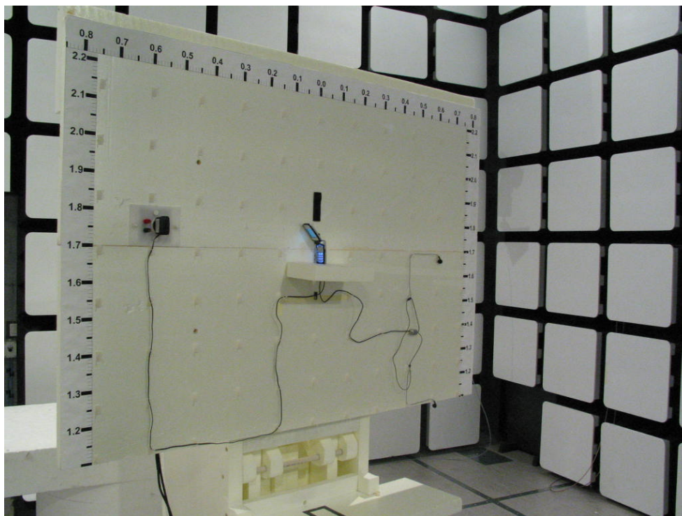
Picture 1 Spurious radiated emission measurement and Bandedge measurement
