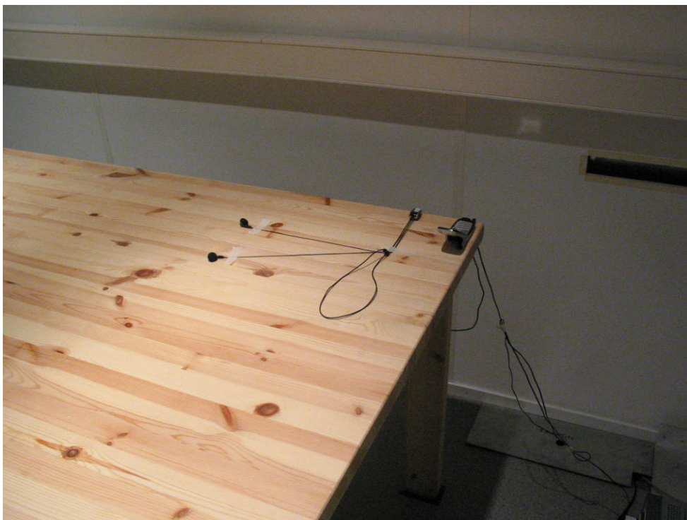
Picture 3 AC powerline conducted emission measurement
