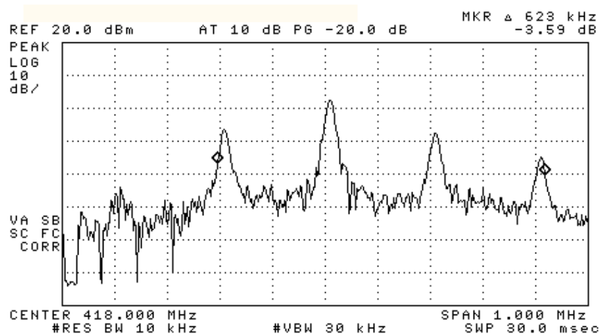
Figure 6: Fundamental Emission Bandwidth.
