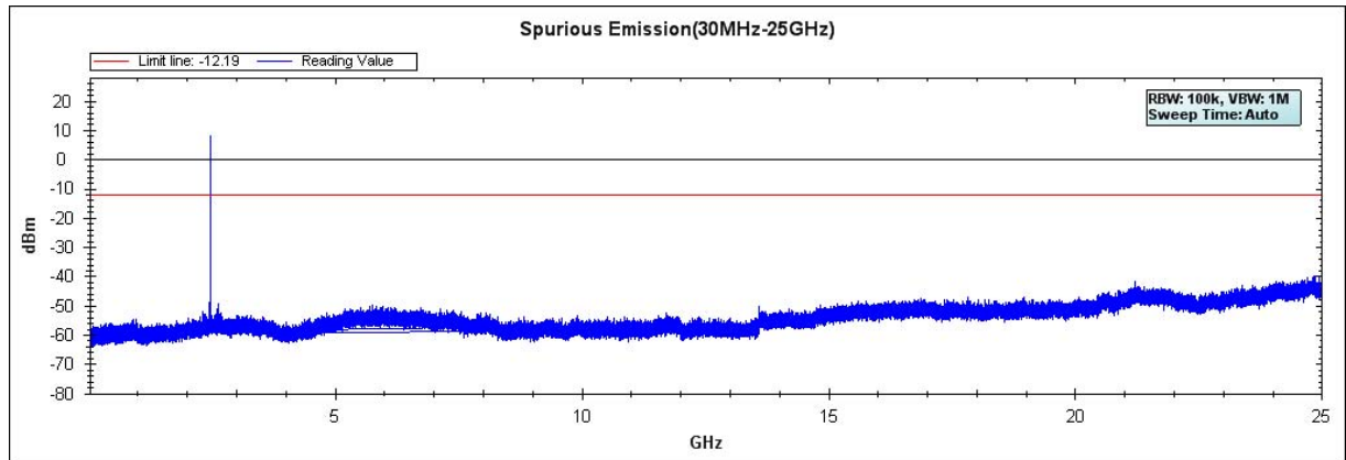
Figure Channel 78: 30MHz-25GHz
