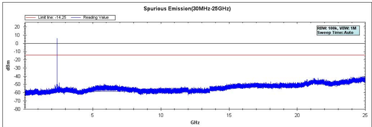
Figure Channel 00: 30MHz-25GHz
