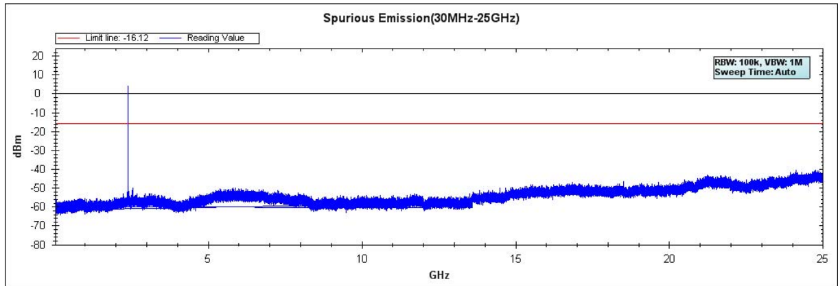
Figure Channel 00: 30MHz-25GHz
