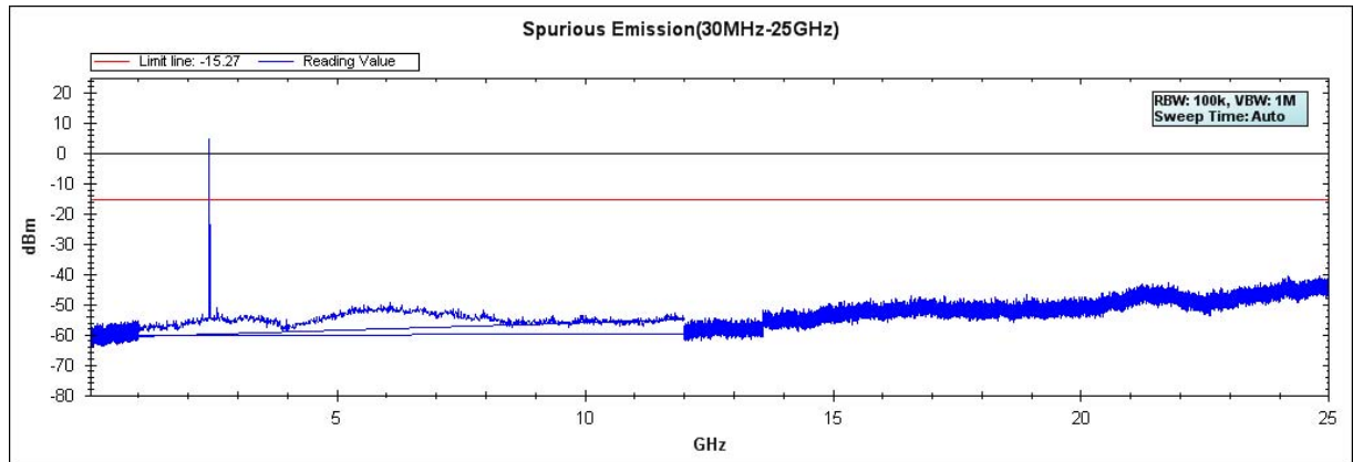
Figure Channel 39: 30MHz-25GHz
