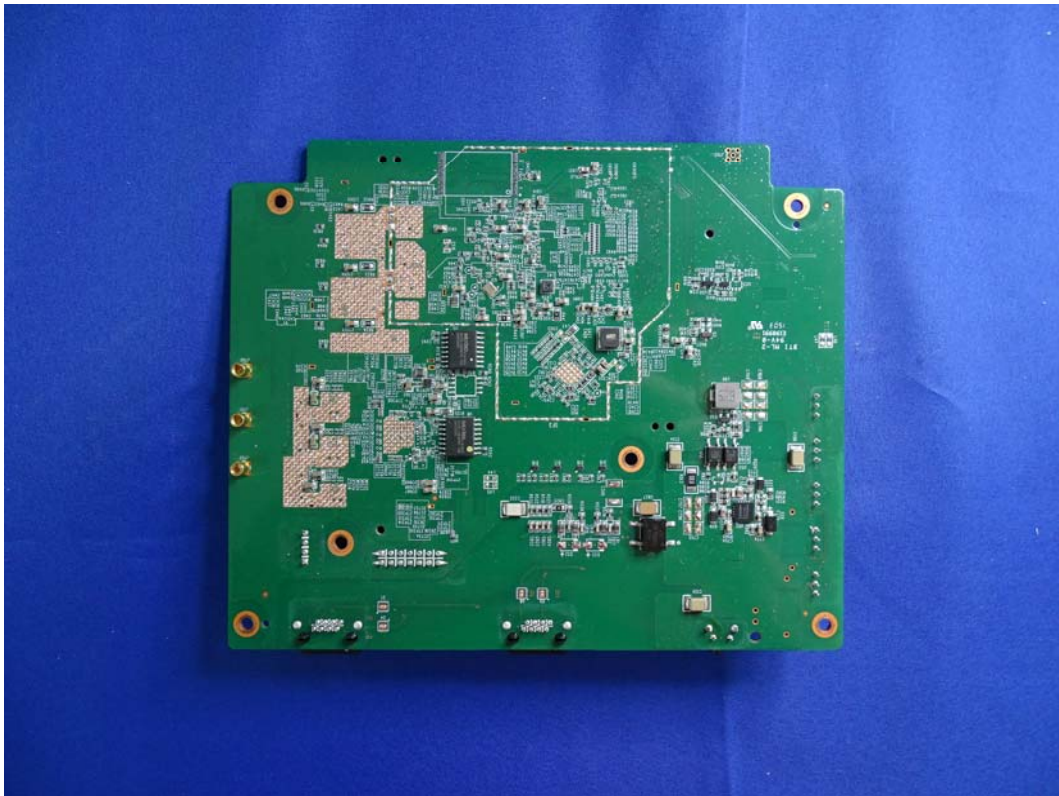
(33) EUT Photo (Internal)
