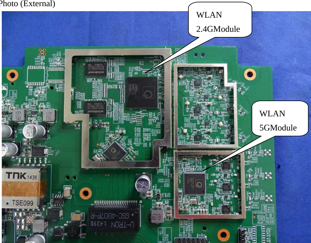
(17) EUT Photo (External)
