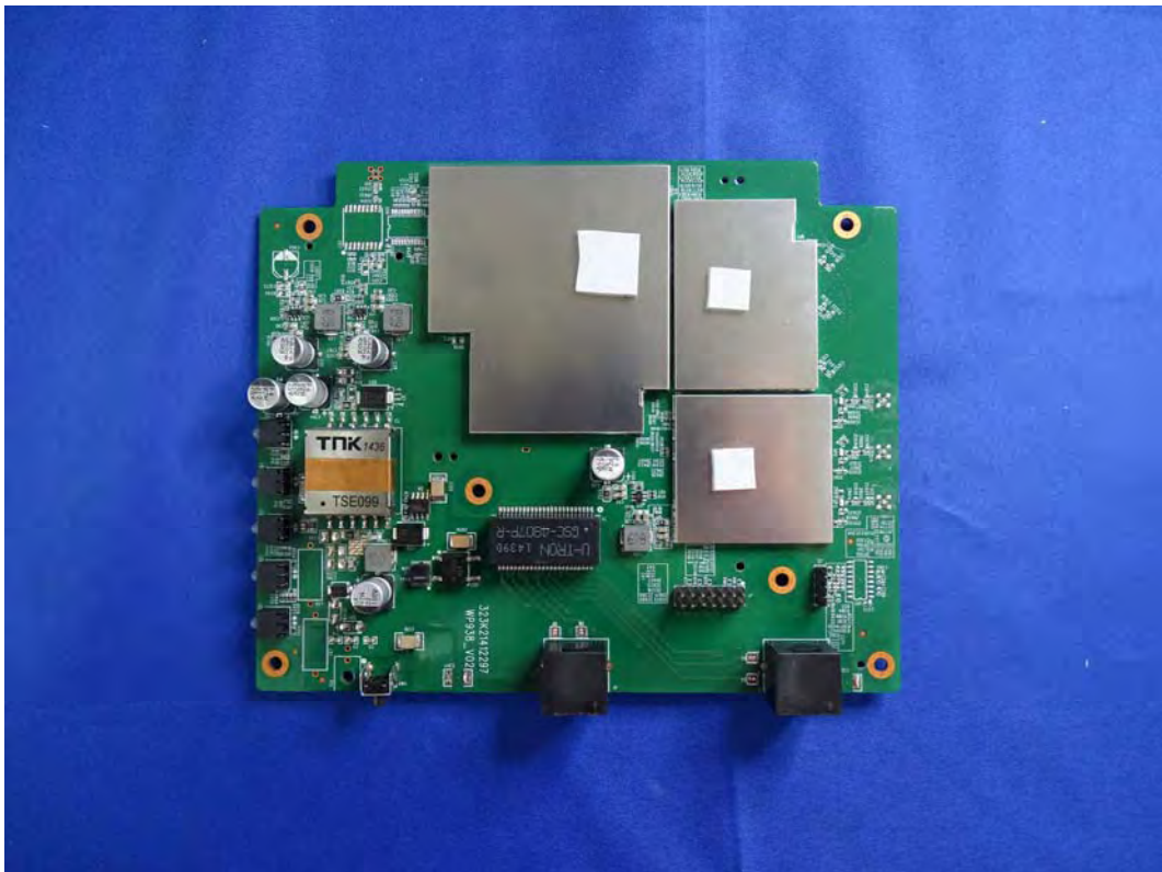
(34) EUT Photo (Internal)
