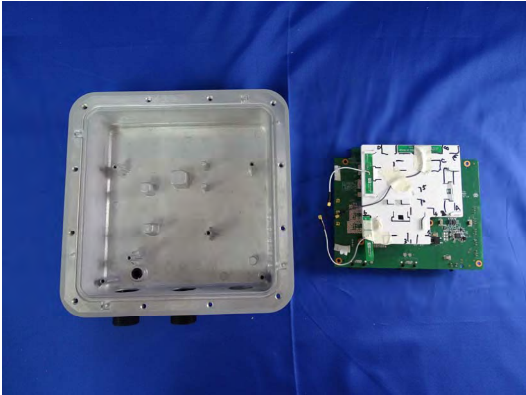
(25) EUT Photo (Internal)
