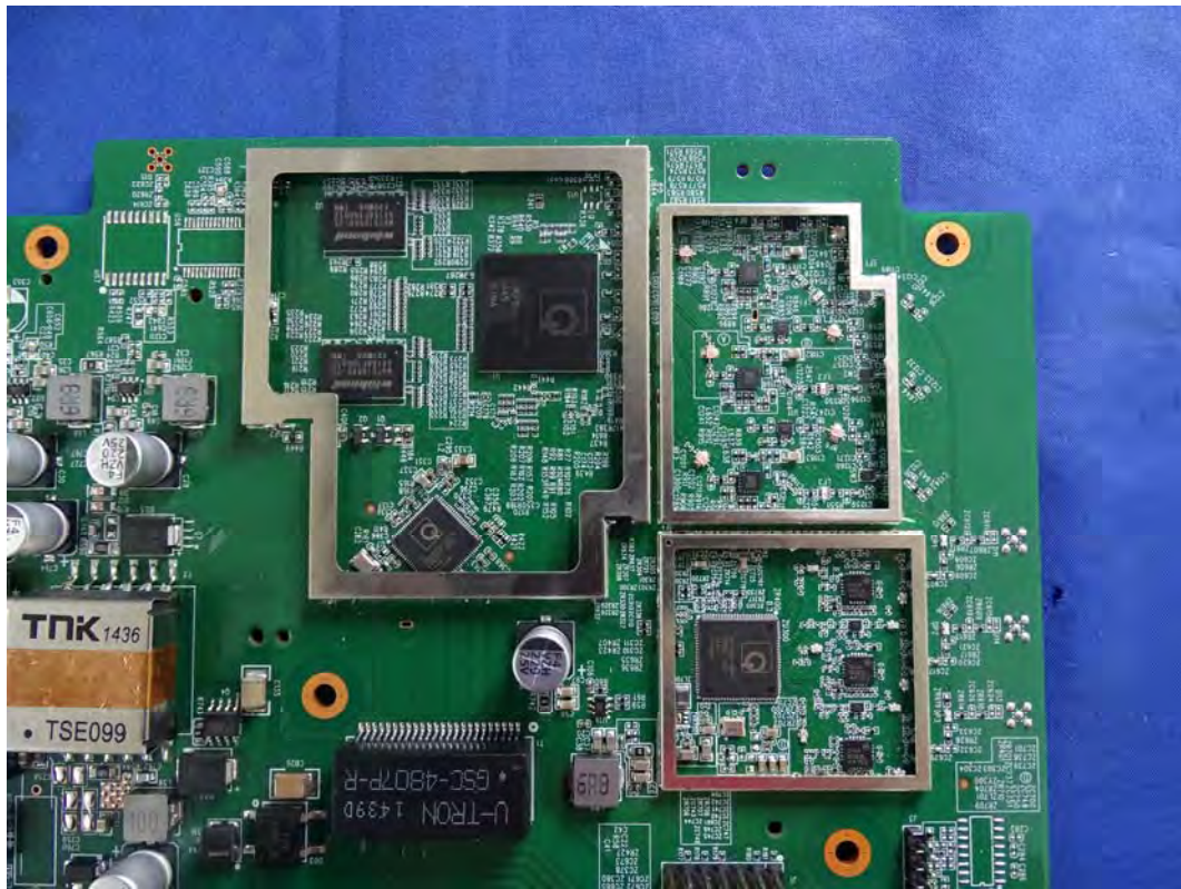
(37) EUT Photo (Internal)
