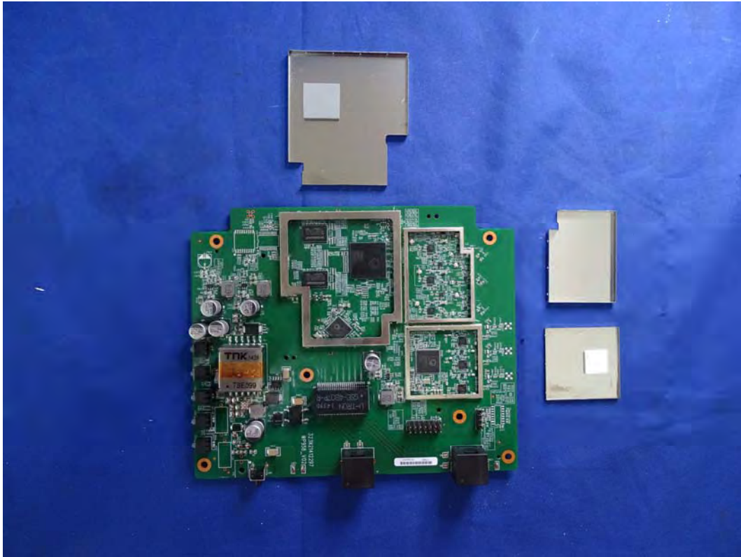
(35) EUT Photo (Internal)
