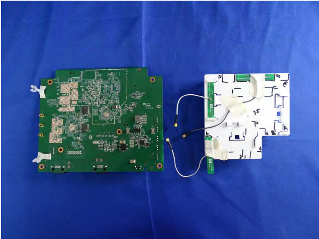
(27) EUT Photo (Internal)
