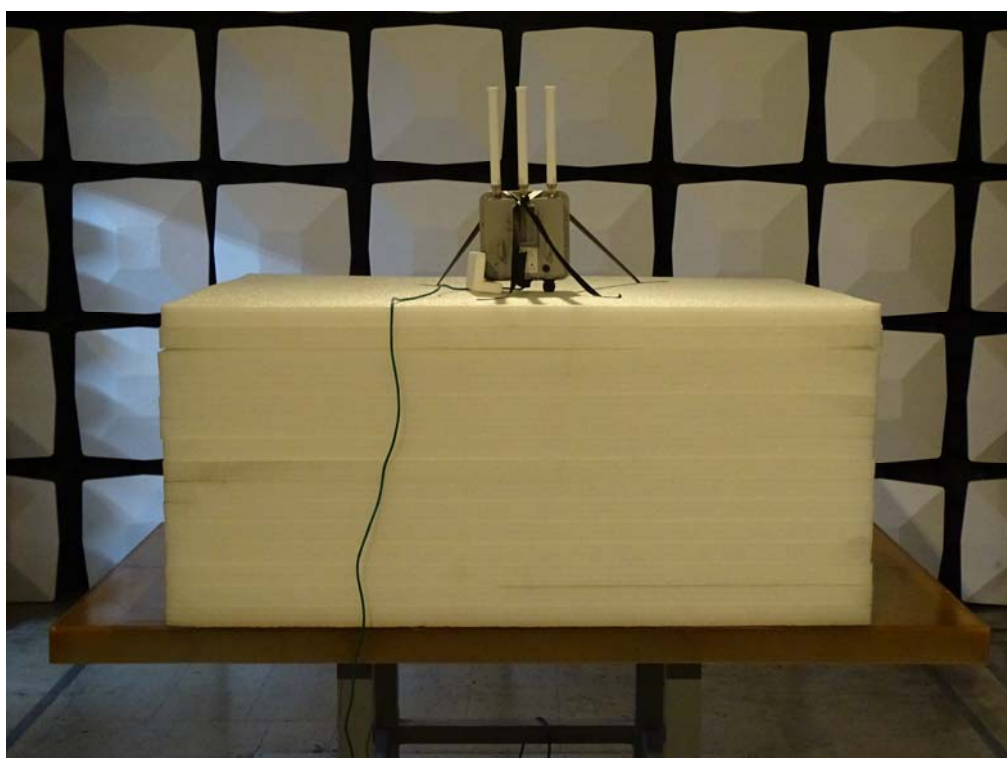
Back View of Radiated Test (Horn) - External
