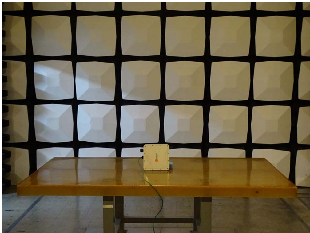
Back View of Radiated Test (Horn) - Internal
