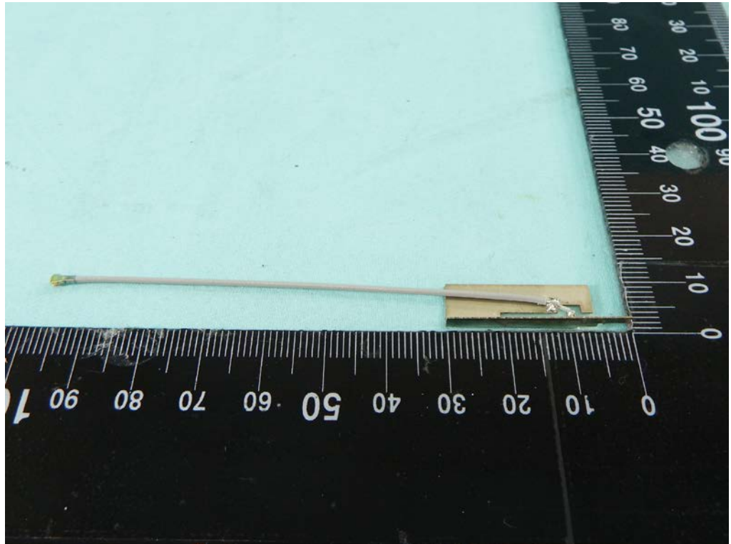
Antenna 7
