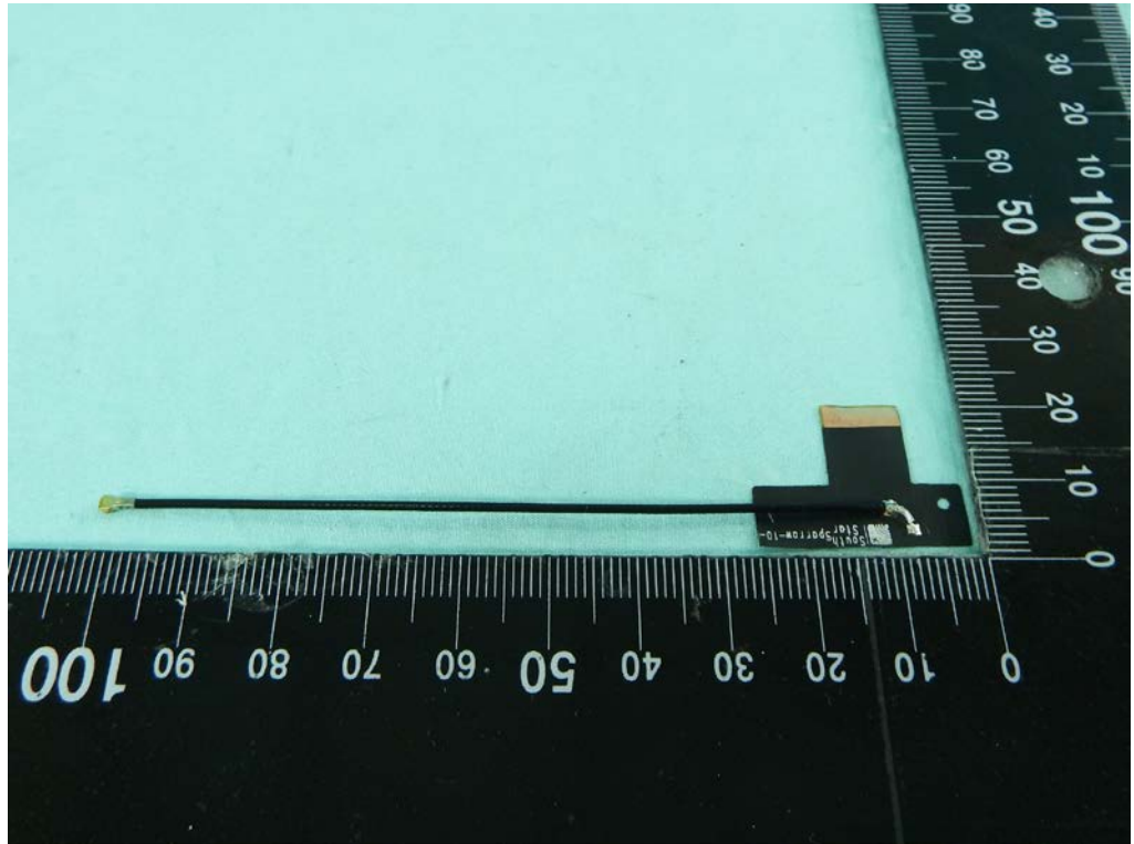
Antenna 4
