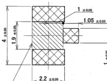
RECOMMENDED FOOTPRINT PATTERN
