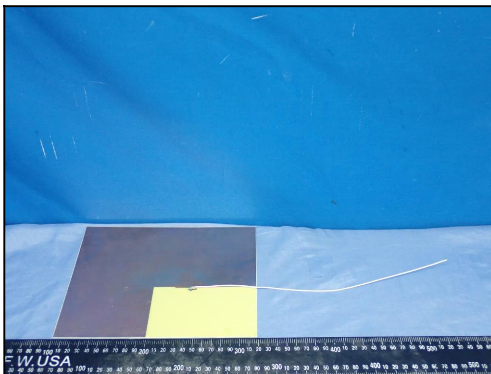
Antenna 2 (Model: 260-25083)
