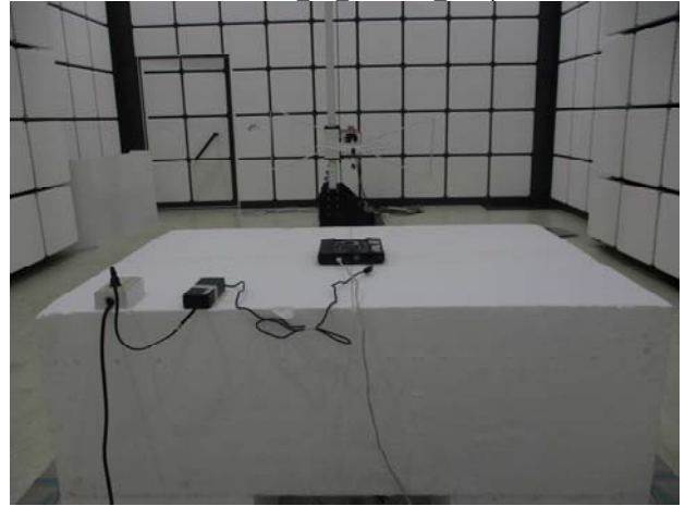
Part 15.247 BT Radiated Setup
