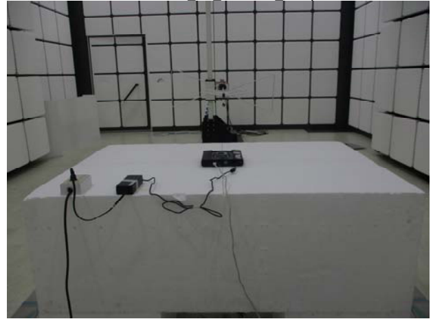
Part 15.407 5G Radiated Setup
