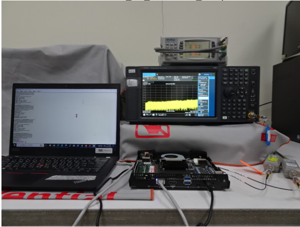
Part 15.407 5G Radiated Setup
