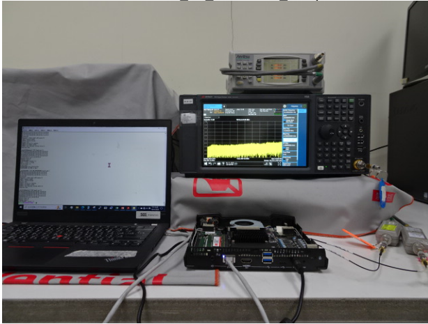
Part 15.247 BT Radiated Setup
