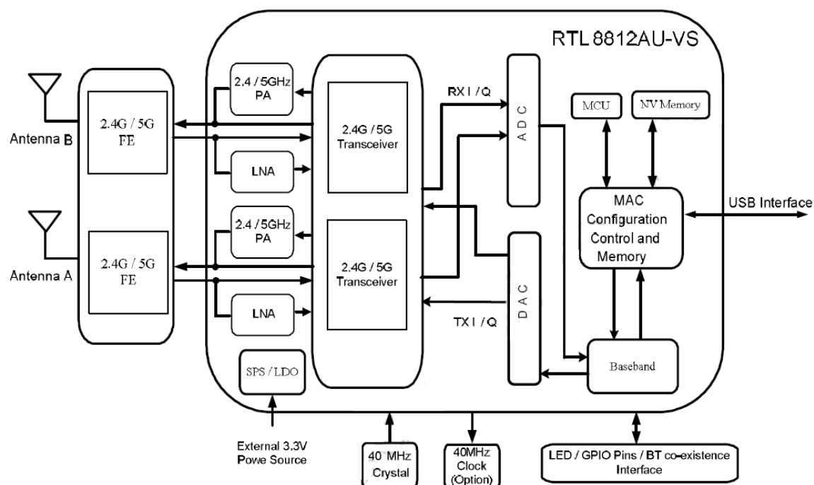
Figure 1. Dual-Band MIMO 2x2 Solution—RTL8812AU-VS (11ac 2x2 MAC/BB/RF + PA)
