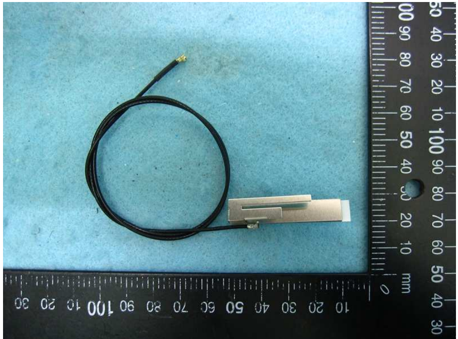
Ant. 3: 450mm
