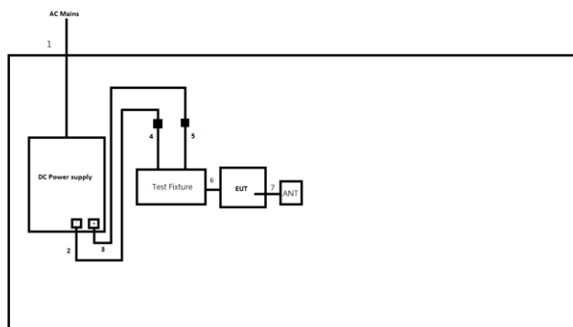
Test Setup Diagram - Radiated Test Dipole Antenna
