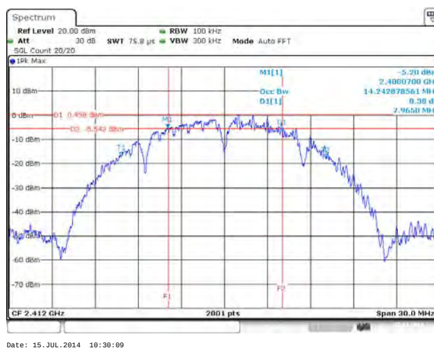
Worst Emission Bandwidth Plots - Chain Port 1
