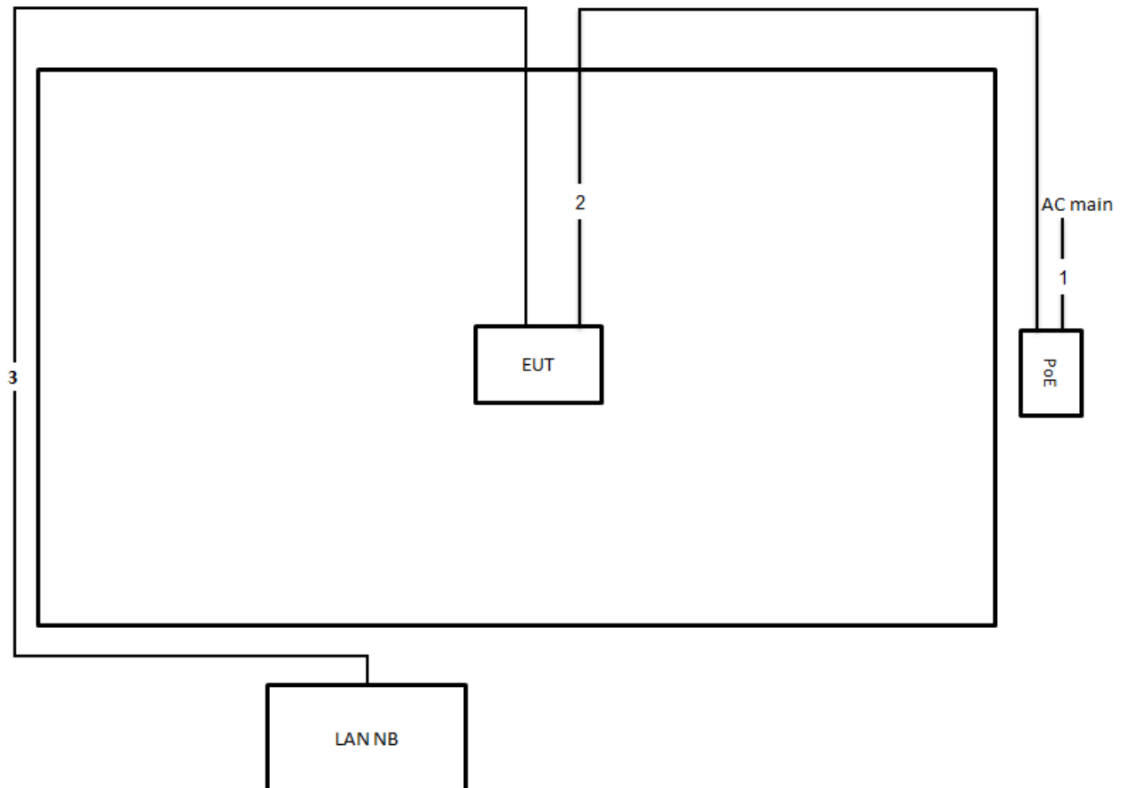
Test Setup Diagram - Radiated Test > 1GHz (for other test items)
