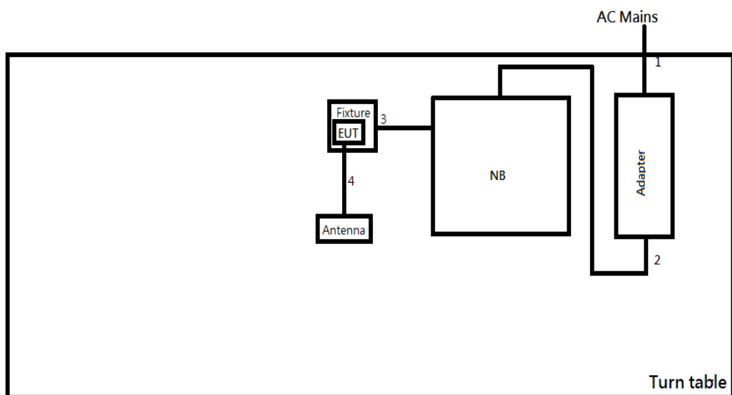
Test Setup Diagram - Radiated Test
