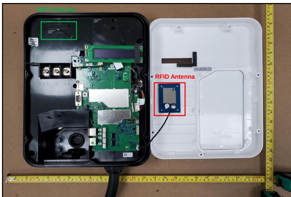
EX-1193-E, EX-1193-E-48
