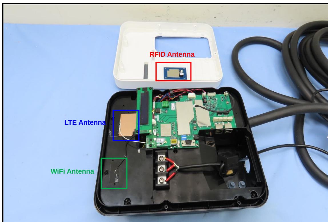
EX-1193-M, EX-1193-M-48
