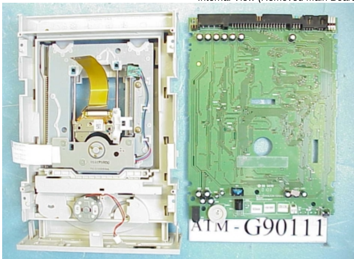
Figure 9 Internal View (Removed Main Board)
