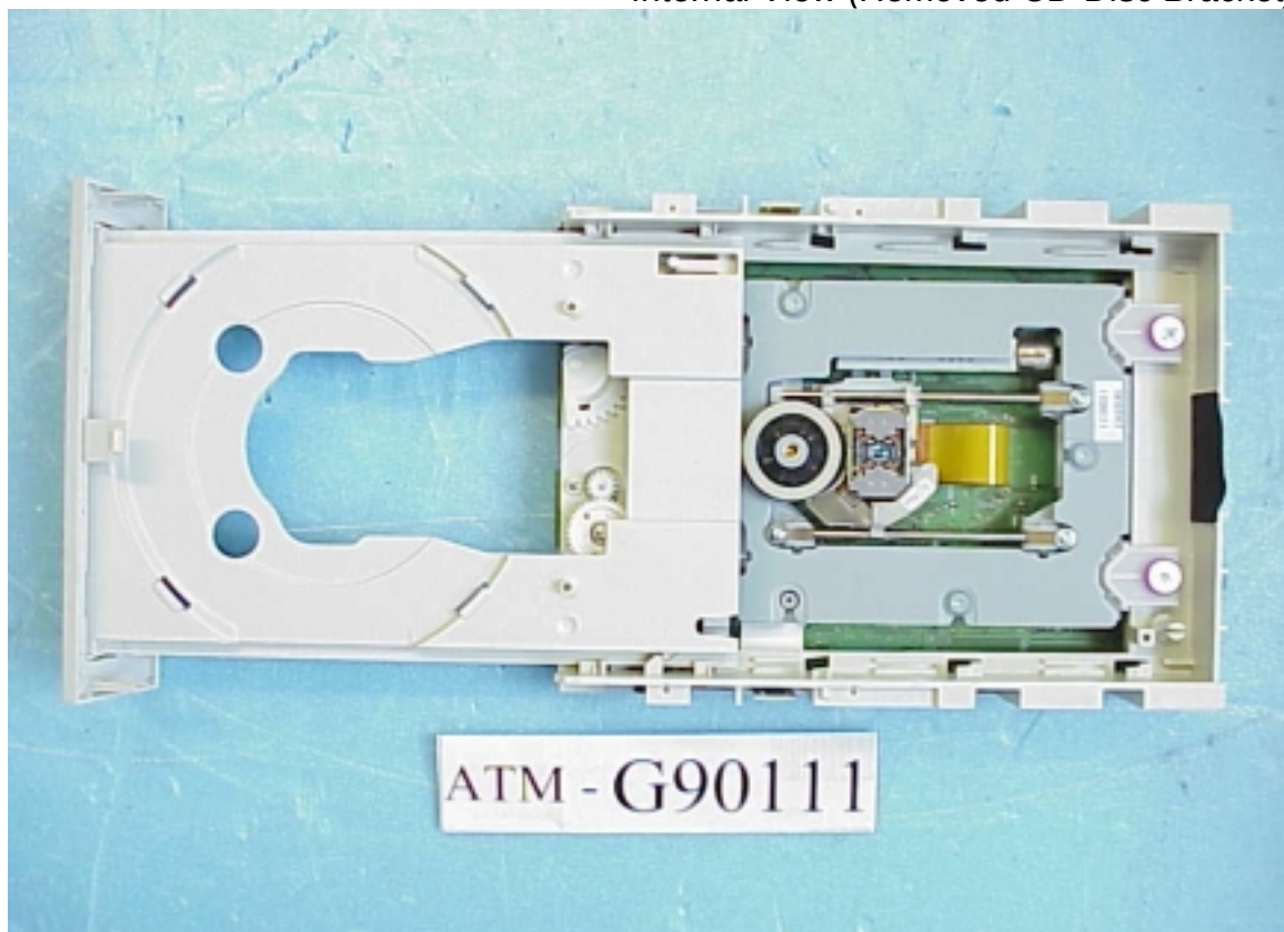
Figure 6 Internal View (Removed CD-Disc Bracket)
