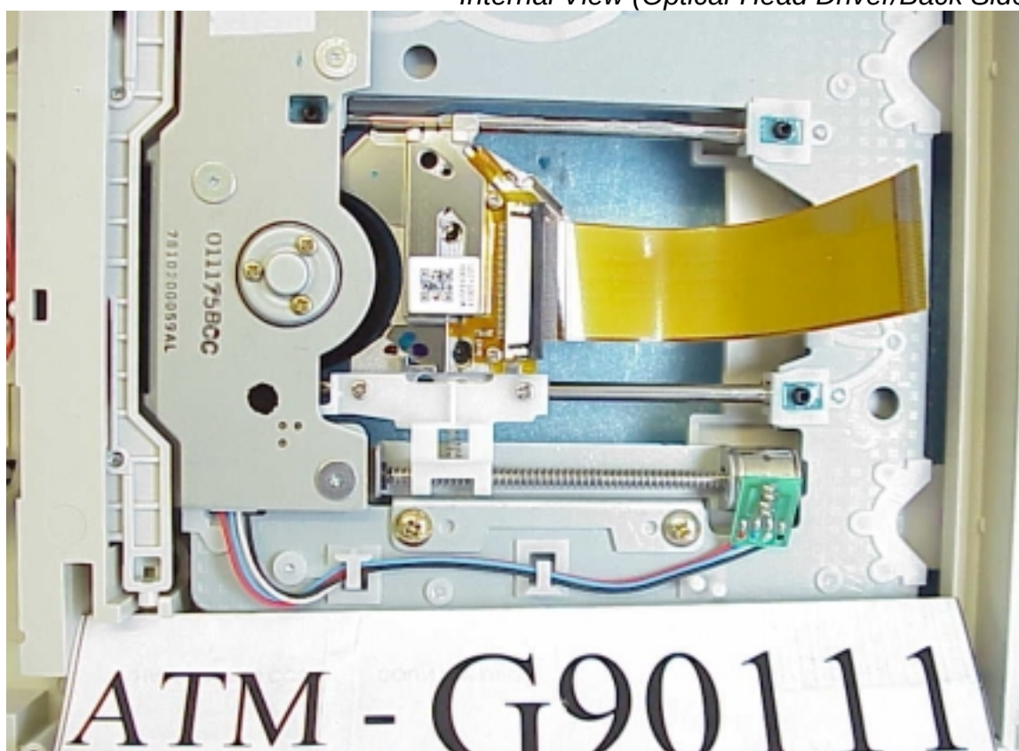
Figure 10 Internal View (Optical-Head Driver/Back Side)
