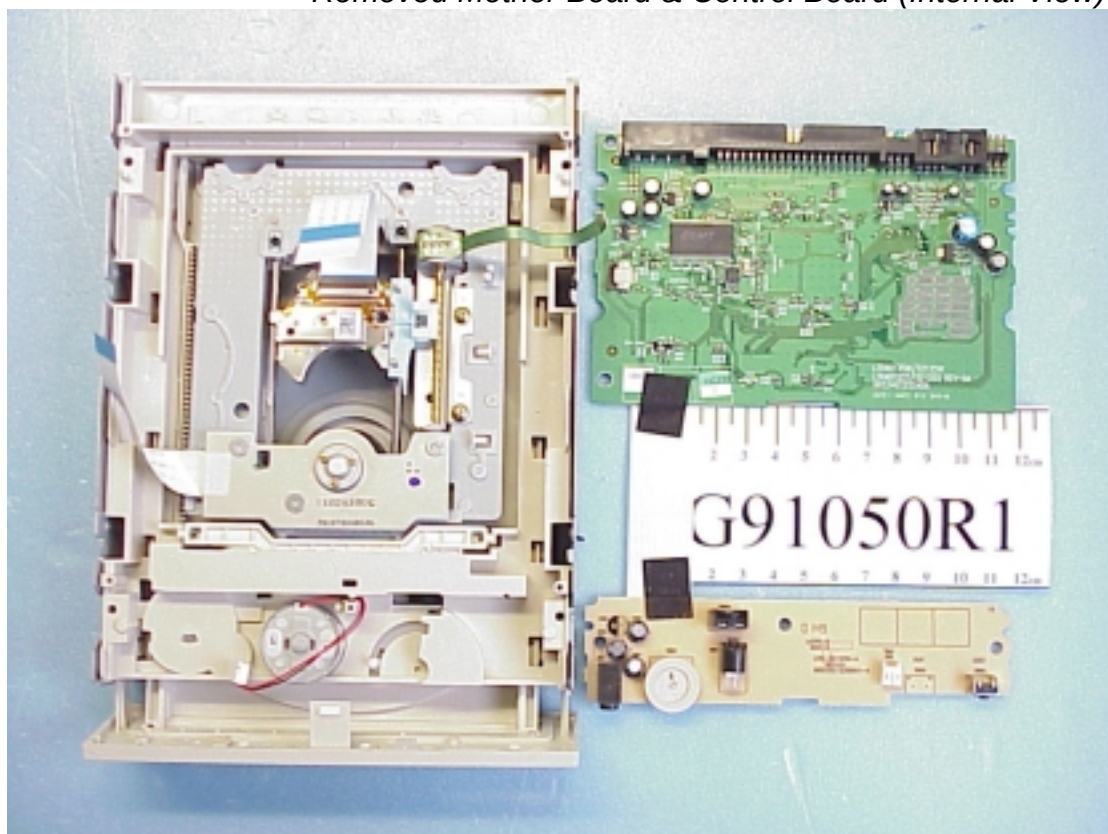
Figure 14 Removed Mother Board & Control Board (Internal View)
