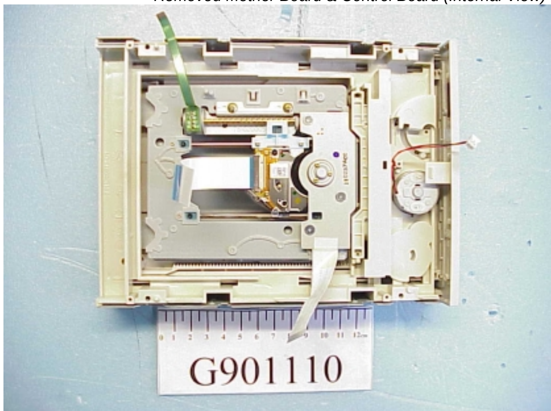
Figure 4 Removed Mother Board & Control Board (Internal View)
