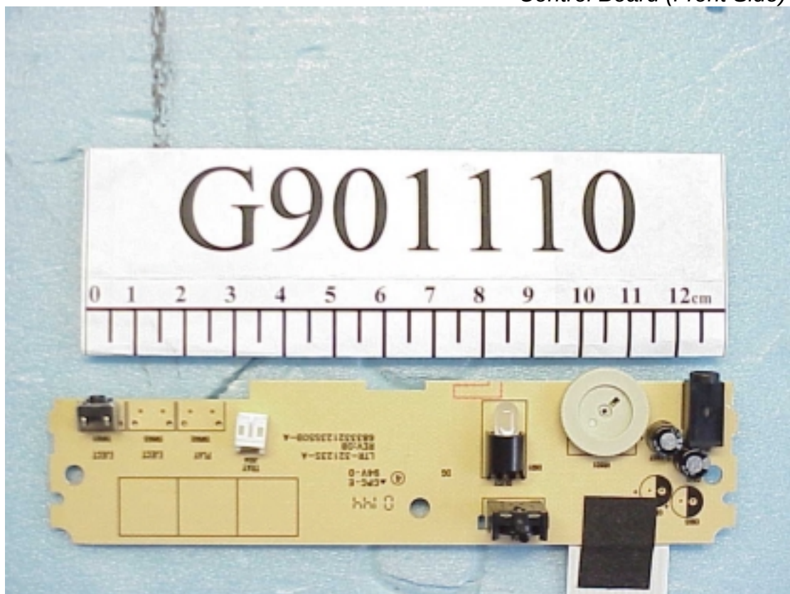
Figure 7 Control Board (Front Side)
