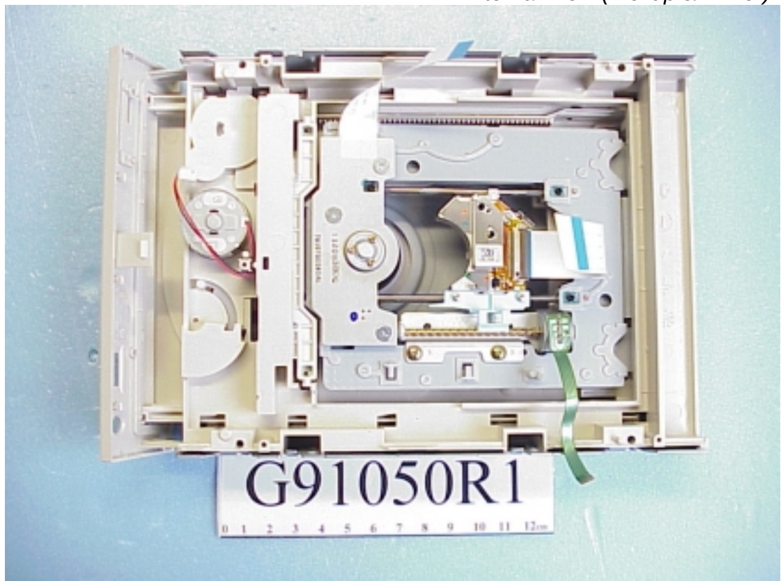
Figure 16 Removed CD-Tray (Internal View)
