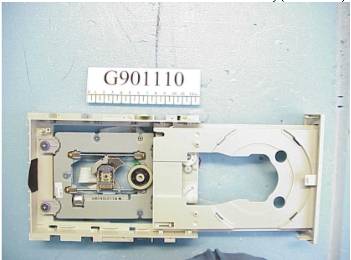
Figure 10 Removed CD-Tray (Internal View)
