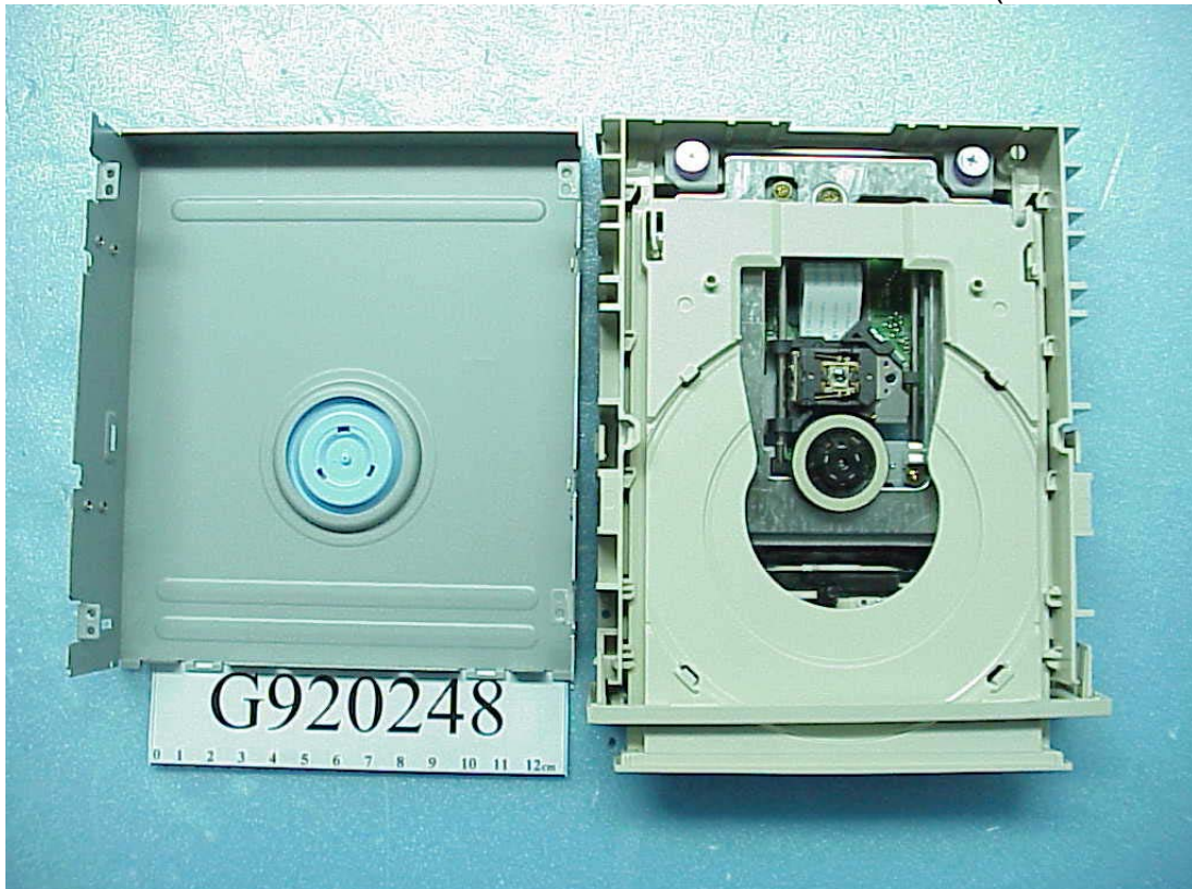
Figure 4 CD-R/RW DRIVE Internal View (Removed Top Case)
