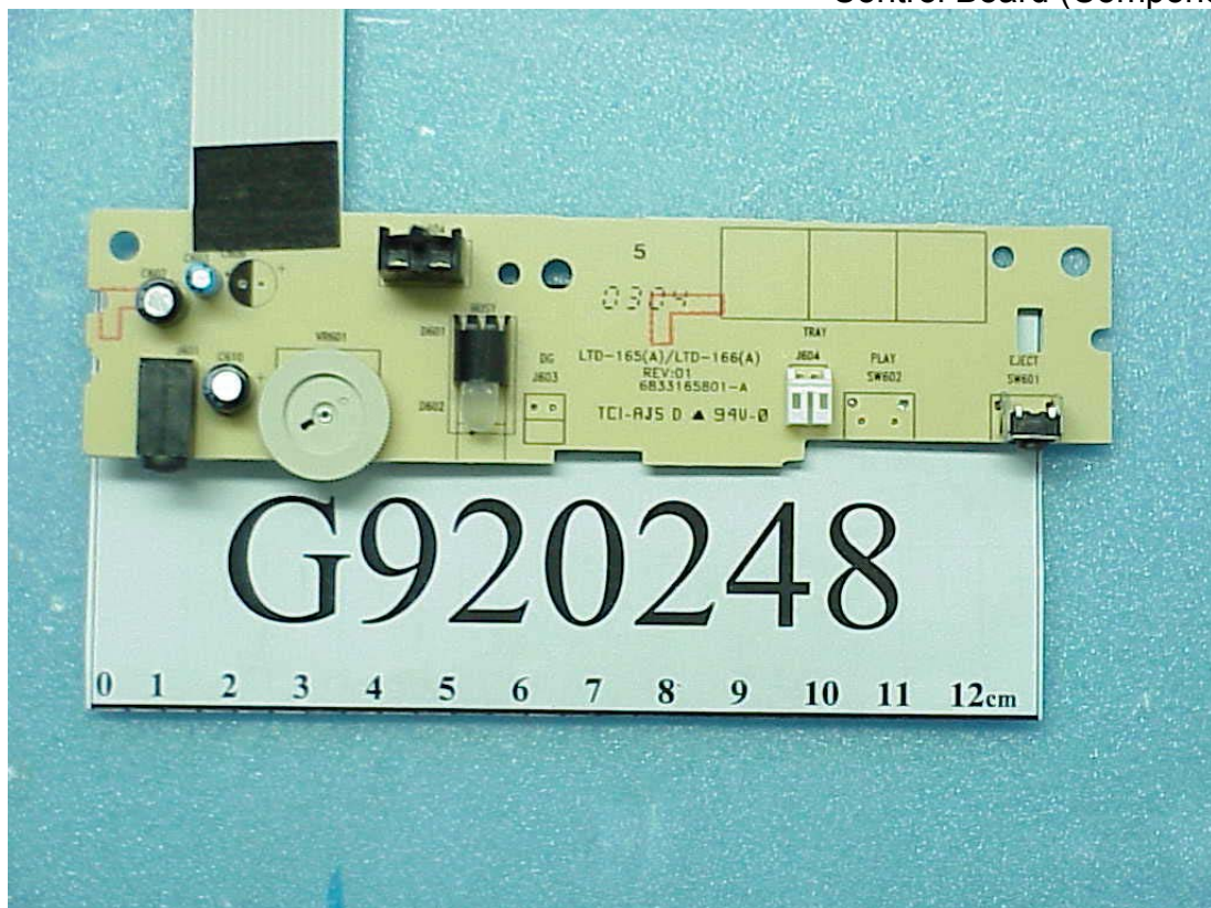
Figure 9 CD-R/RW DRIVE Control Board (Component Side)
