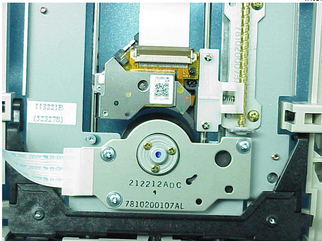
Figure 14 CD-R/RW DRIVE Internal View
