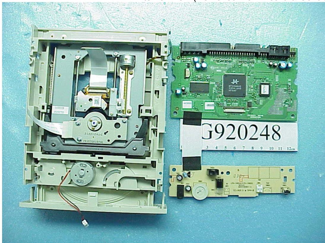
Figure 6 CD-R/RW DRIVE Internal View (Removed Main Board & Control Board)
