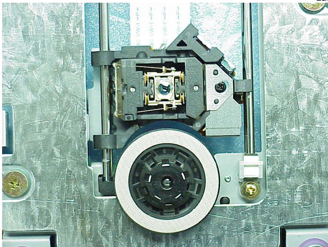
Figure 12 CD-R/RW DRIVE Laser Head
