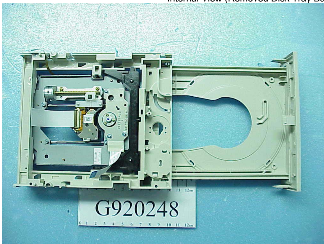
Figure 13 CD-R/RW DRIVE Internal View (Removed Disk Tray Back View)
