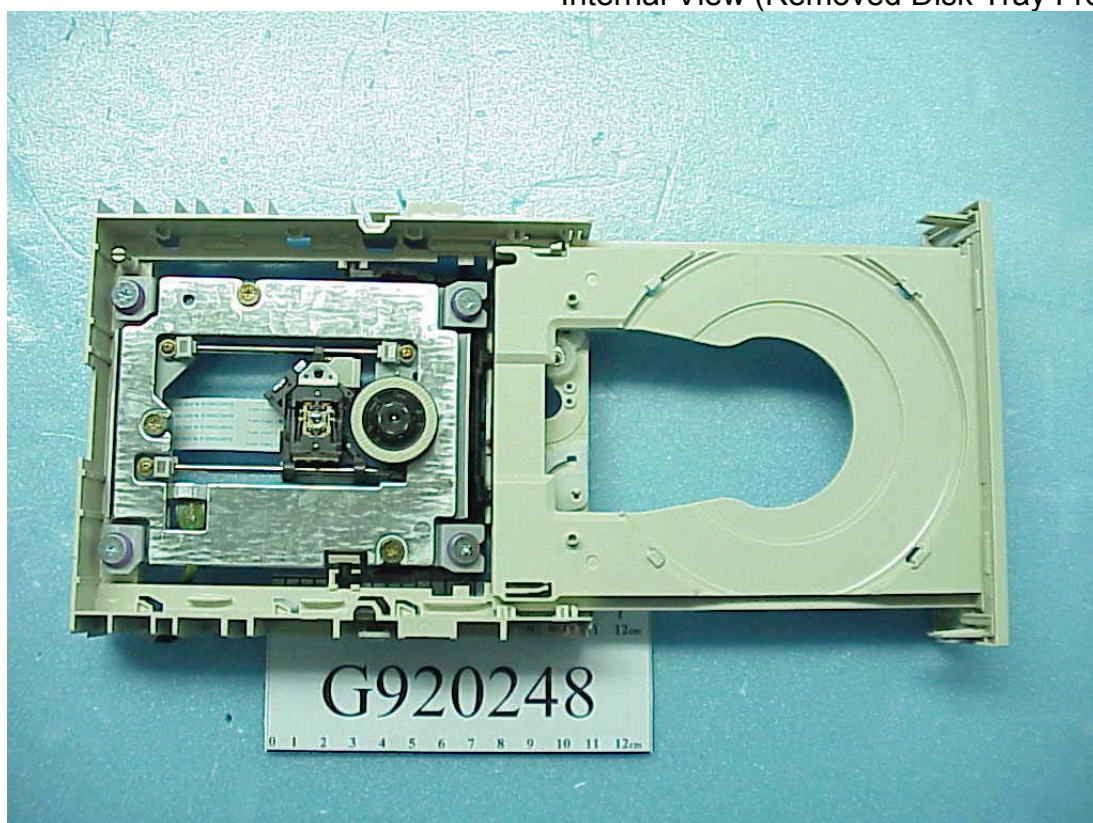
Figure 11 CD-R/RW DRIVE Internal View (Removed Disk Tray Front View)
